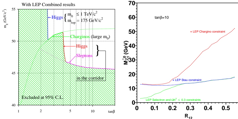
Figure 3. Mass limit on the \tilde{\chi}_1^0 including Chargino, Higgs and sleptons searches at LEP 5 (left side) and when relaxing the gaugino mass unification at the GUT scale 7 (right side)
