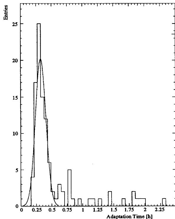
Figure 9: Distribution of adaptation times after temperature changes in steps of 5^{\circ}\text{C} .
