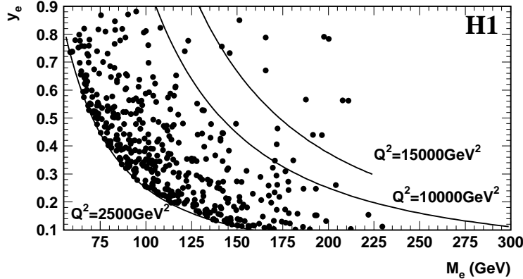
Figure 3: Selected NC DIS candidate events in the M_e - y_e plane; three contours of fixed Q^2 are shown.
