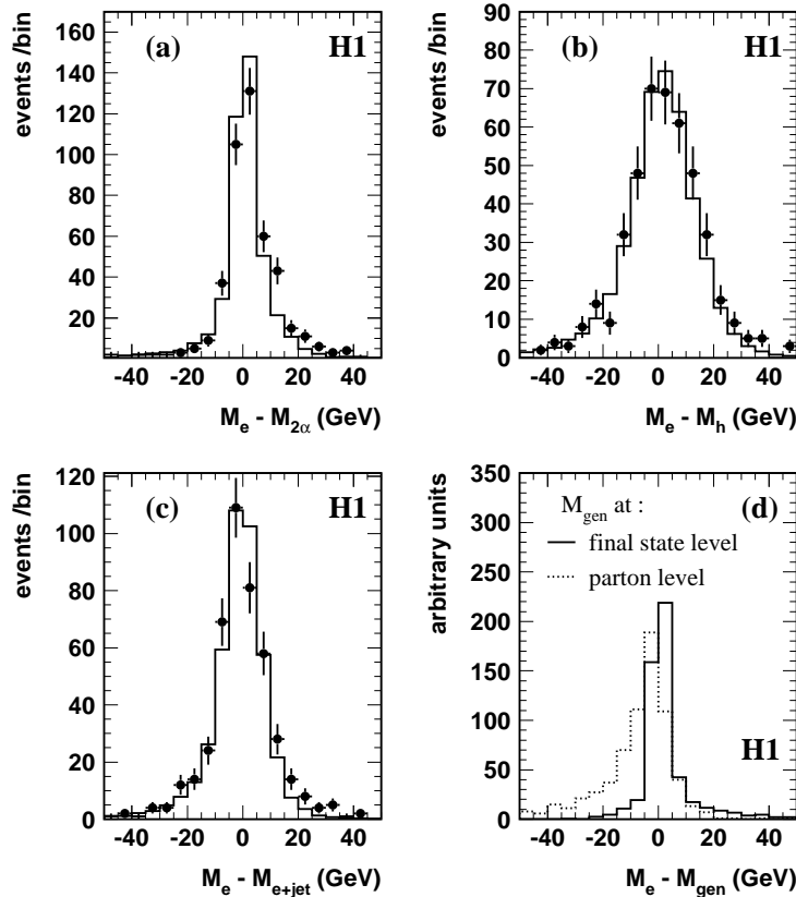
Figure 2: Distributions for the NC DIS sample of the differences between the mass ( M = \sqrt{xs} ) calculated using the e -method ( M_e ) and (a) using the 2\alpha -method ( M_{2\alpha} ), (b) using the h -method ( M_h ), and (c) using the invariant mass of the positron-jet system ( M_{e+jet} ); superimposed on the data points ( \bullet symbols) are histograms of the expectation from the Monte Carlo simulation; (d) difference between M_e and the generated mass M_{gen} when the latter is calculated either from the final state positron using simulated NC DIS events (histogram), or taken from the invariant mass of the positron-quark sub-system in a specific eq resonance model (dotted histogram).
