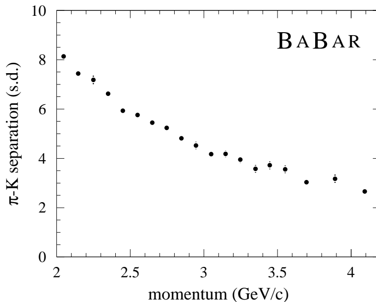
Figure 10: DIRC \pi -K separation versus track momentum measured in D^0 \rightarrow K^- \pi^+ decays selected kinematically from inclusive D^* production.
