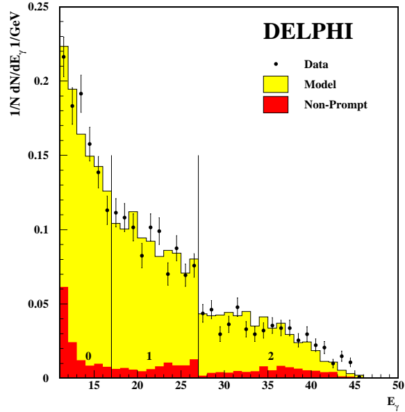
Figure 2: The energy distribution of the selected isolated photon events. The three classes (0,1,2) correspond to a mean centre-of-mass energy of 76, 66 and 45 GeV, respectively. The steps between the classes result from different \pi^0 rejection cuts.
