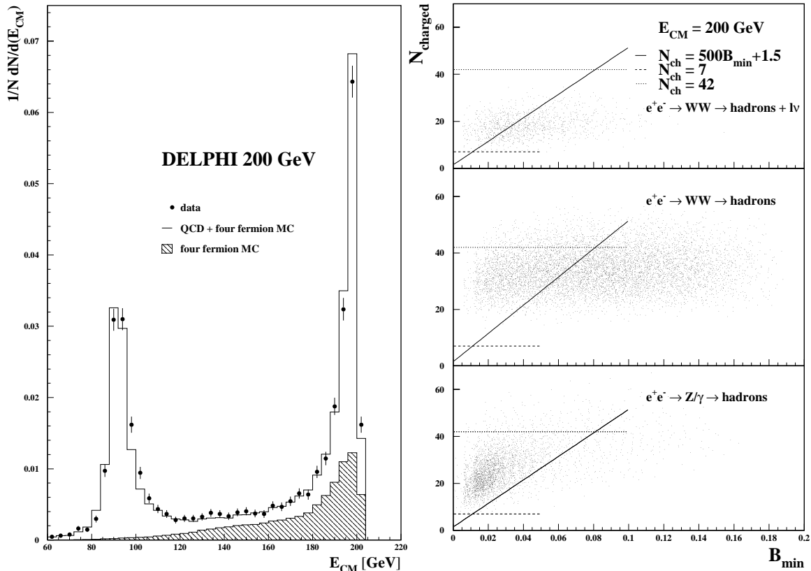
Figure 1: Left: Reconstructed centre-of-mass energy for accepted data before \sqrt{s'} cut compared to QCD and four-fermion simulation. Right: Simulation of four-fermion background and QCD events in the N_{\text{ch}}-B_{\text{min}} plane. The upper two plots show the distributions for semi-leptonic and fully hadronic WW events, respectively. The lines indicate the cut values chosen.
