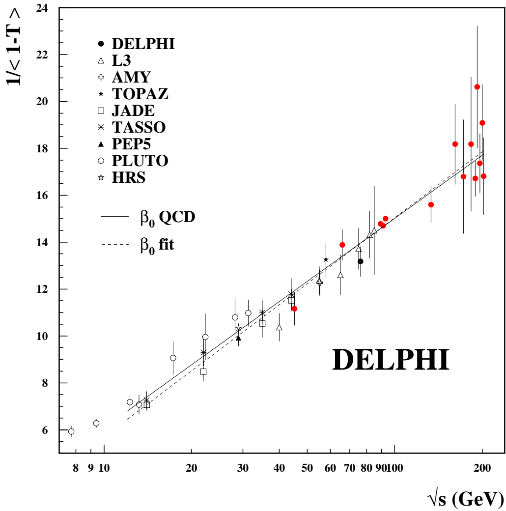
Figure 17: The running of 1/(1-T) against \log(E_{cm}) . The results of the theoretical prediction and a combined fit of the data of several experiments is shown.
