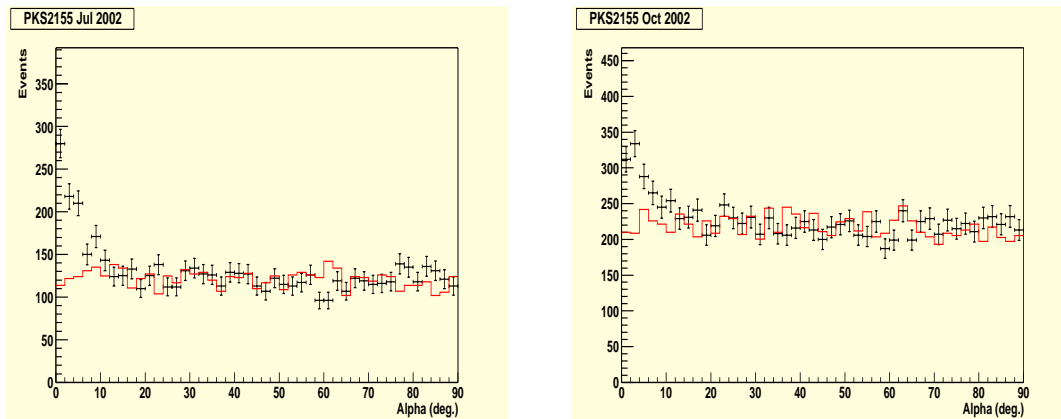
Fig. 1. The pointing angle \alpha -plot of PKS 2155-304 observations for July (left panel) and October (right panel) 2002. The OFF-source distributions have been normalised to the control region between 30^\circ and 90^\circ .
