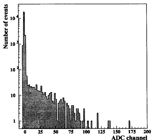
Fig. 4. A LED run for 2” photo tubes. The peak at 0 corresponds to “0” photo-electron.
