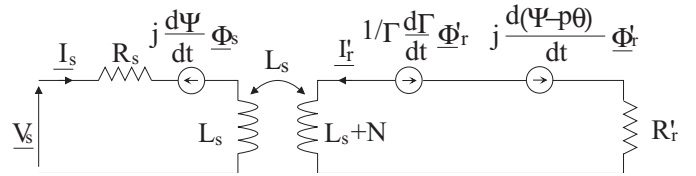
Fig. 12. Two-phase saturated model with leakage inductance totaled in the rotor.
