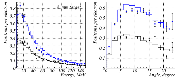
Figure 3: The energy and angular spectra corrected by efficiency for the 8 mm target. E^- = 6 GeV. Boxes — crystal, points — amorphous target. Histograms — corresponding simulation.
