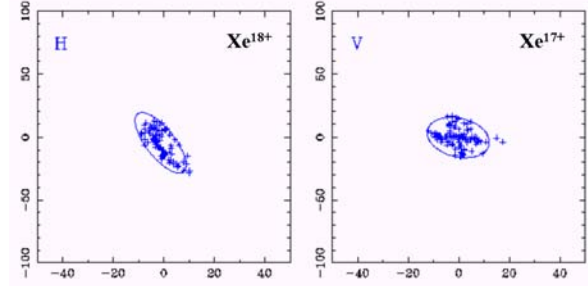
Fig. 7 : Simulation results of the Xe 18+ and Xe 17+ emittances fitting experimental beam constraints.
