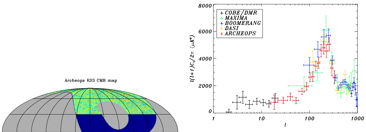
Figure 2: Left : ARCHEOPS CMB map (Galactic coordinates, centered on the Galactic anticenter, Northern hemisphere) in HEALPIX pixelisation with 15 arcmin. pixels and a 15 arcmin. Gaussian smoothing. The map is a two-photometers coaddition. The dark blue region is not included in the present analysis because of possible contamination by dust. The colors in the map range from -500 to 500\mu\text{K}_{\text{CMB}} . Right : The ARCHEOPS power spectrum compared with results of COBE, Boomerang, Dasi, Maxima.
