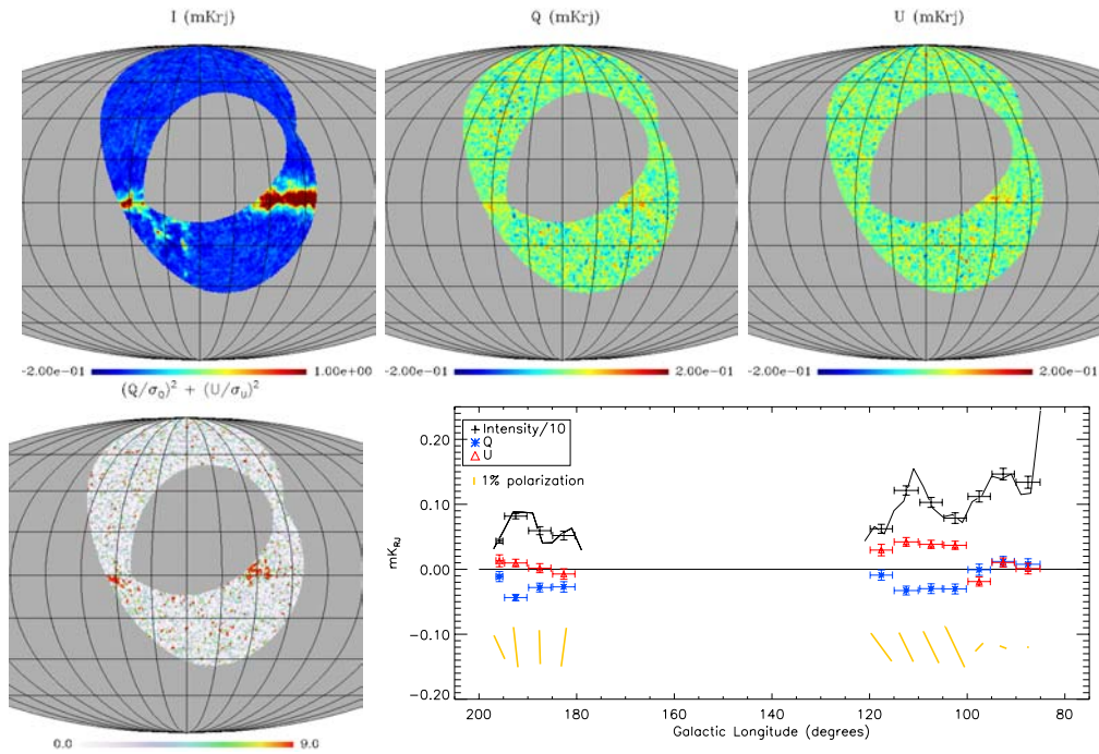
Figure 4: Top left: Map of Intensity at 353 GHz. Top center: Map of Q Stokes parameter. Top right: Map of U Stokes parameter. Bottom left: Map of the normalized squared polarized intensity (Q^2 + U^2)/(\sigma_Q^2 + \sigma_U^2) . Twice this quantity is statistically distributed like a \chi^2 with 2 degrees of freedom. The 68, 95.4, 99.7% CL of the mapped quantity correspond to 1.1, 3.1, 5.8 respectively. Bottom right: Summary figure of diffuse Galactic polarization. The intensity (divided by 10) is represented in black and is taken to be the average value for -2 \leq b \leq 2 in each longitude band. The thin solid line is the same value in 2^\circ wide bands. The direction of polarization for every bin is represented below in gold, and the length of the dash is proportional to the degree of polarization p in %. The horizontal error bars represent the width of the longitude bins, which is 5^\circ except for the edge bins.
