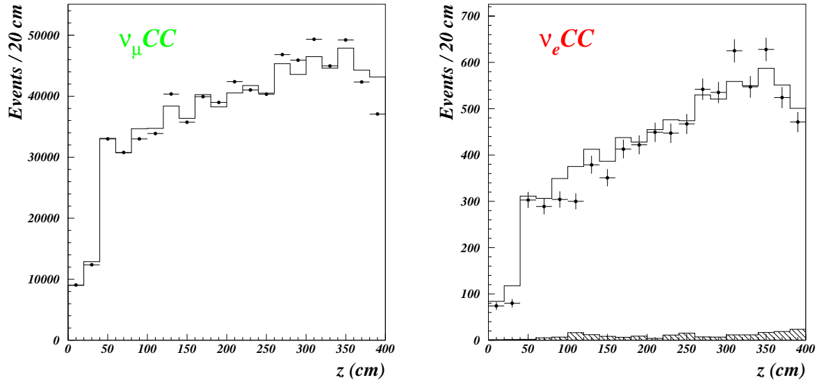
Figure 3: The distributions of z (defined in the text) for \nu_\mu CC (left) and \nu_e CC (right) candidates in the data (points with error bars) and in the Monte Carlo (histogram). The Monte Carlo distribution of \nu_\mu CC events is normalized to the number of \nu_\mu CC events in the data; the Monte Carlo distribution of \nu_e CC events is normalized using the relative \nu_e CC/ \nu_\mu CC abundance predicted by our simulation. The background contribution to the \nu_e CC sample is shown in the hatched histogram.
