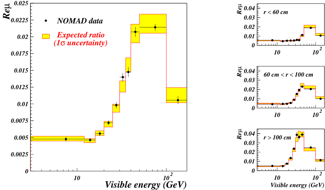
Figure 7: The R_{e\mu} ratio as a function of the visible energy for the data (points) and for the Monte Carlo prediction assuming no oscillations (filled bands), for the full radial acceptance (left) and in the three radial bins (right). The upper and lower boundaries of the bands correspond to the predictions with \pm 1\sigma uncertainty, where \sigma includes both the normalization and energy-dependent systematic uncertainties added in quadrature.
