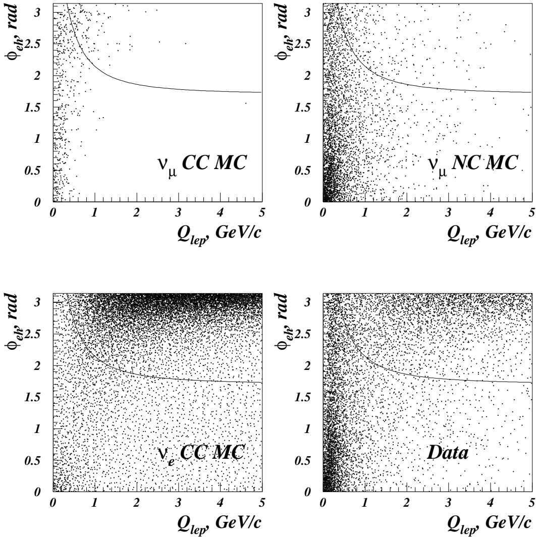
Figure 2: The two-dimensional distributions \phi_{eh} - Q_{lep} (defined in the text) for Monte Carlo \nu_{\mu} CC and \nu_{\mu} NC (background) events and for \nu_e CC (signal) events, as well as for the NOMAD data. The events to the right of the curve were selected.
