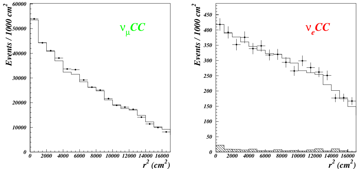
Figure 5: The distribution of r^2 , the square of the radial position of the neutrino interaction vertex with respect to the nominal beam axis, for the data (points with error bars) and the Monte Carlo (histogram), for \nu_\mu CC (left) and \nu_e CC (right) candidates. The normalization of the Monte Carlo distributions is the same as in the two previous plots. The background contribution to the \nu_e CC sample is shown in the hatched histogram.
