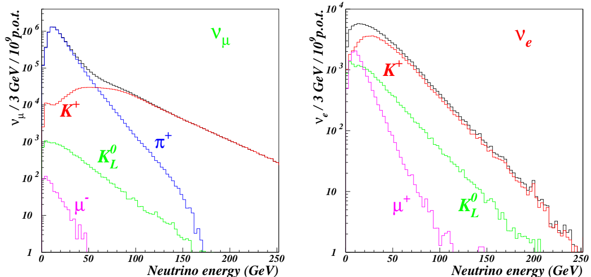
Figure 1: Composition of the \nu_\mu and \nu_e energy spectra at NOMAD, within a transverse fiducial area of 260 \times 260 \text{ cm}^2 , as predicted by the NOMAD simulation of the neutrino beam line.
