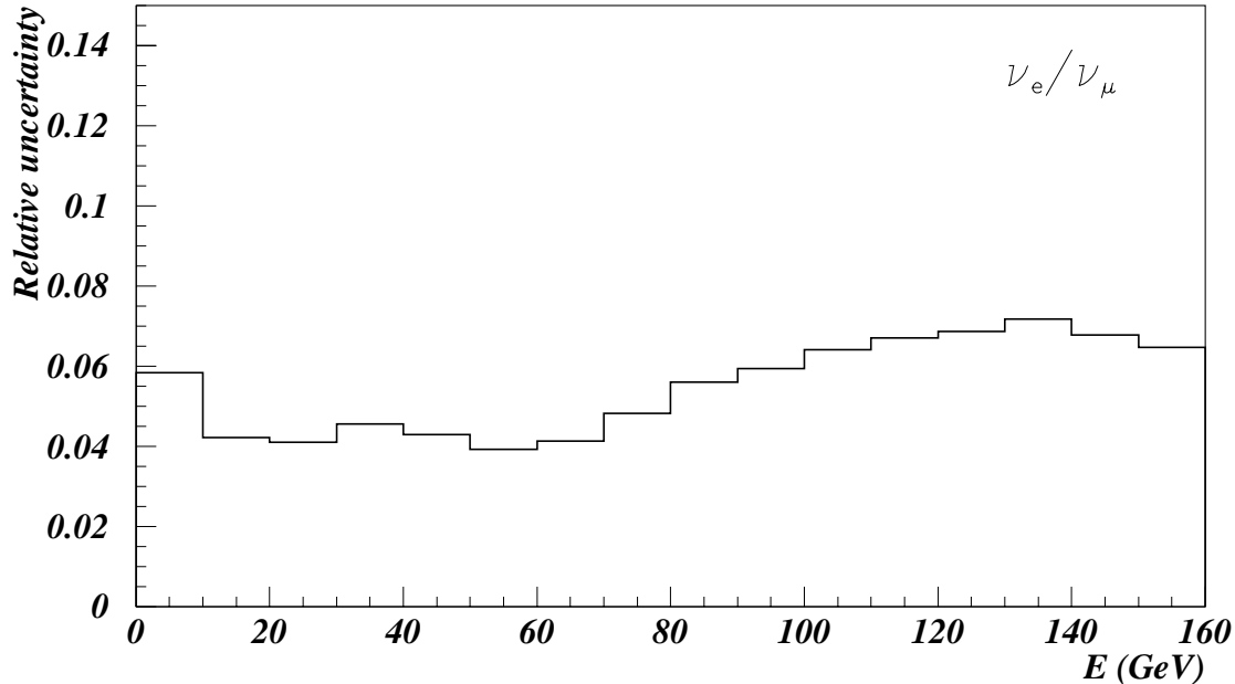
Figure 6: Energy-dependent uncertainty in the prediction of the R_{e\mu} ratio.
