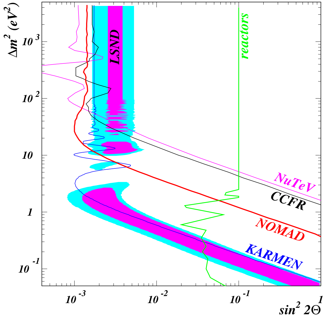
Figure 8: The 90% C.L. exclusion region in the \Delta m^2 - \sin^2(2\theta) plane from this analysis superimposed on the results of other experiments.
