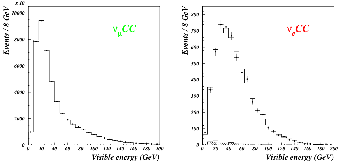
Figure 4: Neutrino energy spectra for the data (points with error bars) and the Monte Carlo (histogram), for \nu_\mu CC (left) and \nu_e CC (right) candidates. The normalization of the Monte Carlo distributions is the same as in Fig. 3. The background contribution to the \nu_e CC sample is shown in the hatched histogram.
