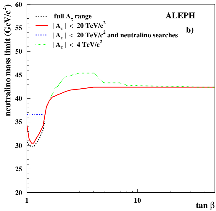
Figure 6: Limits on the mass of the lightest neutralino as a function of (a) |\tan \phi_\tau| and (b) \tan \beta .
