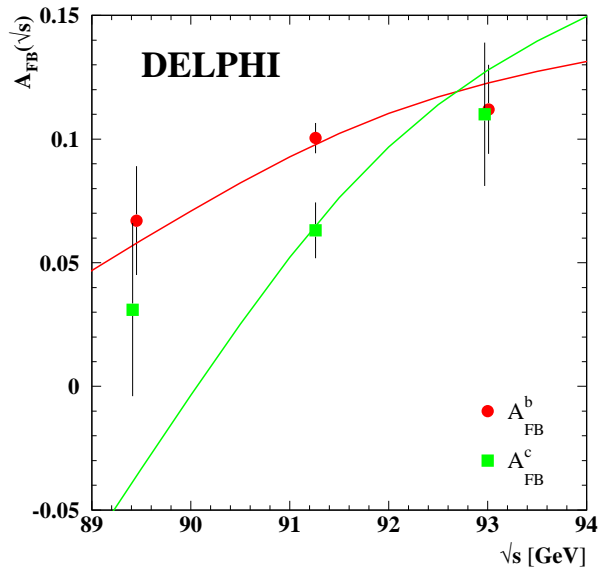
Figure 5: Measured values of A_{\text{FB}}^{(b)} and A_{\text{FB}}^{(c)} at different \sqrt{s} compared to the Standard Model predictions for m_t = 175 \text{ GeV}/c^2 and m_H = 300 \text{ GeV}/c^2 . (To avoid the overlap of the results at peak-2 and peak+2, the A_{\text{FB}}^{(b)} and A_{\text{FB}}^{(c)} points have been shifted respectively by +0.02 \text{ GeV} and -0.02 \text{ GeV} .)
