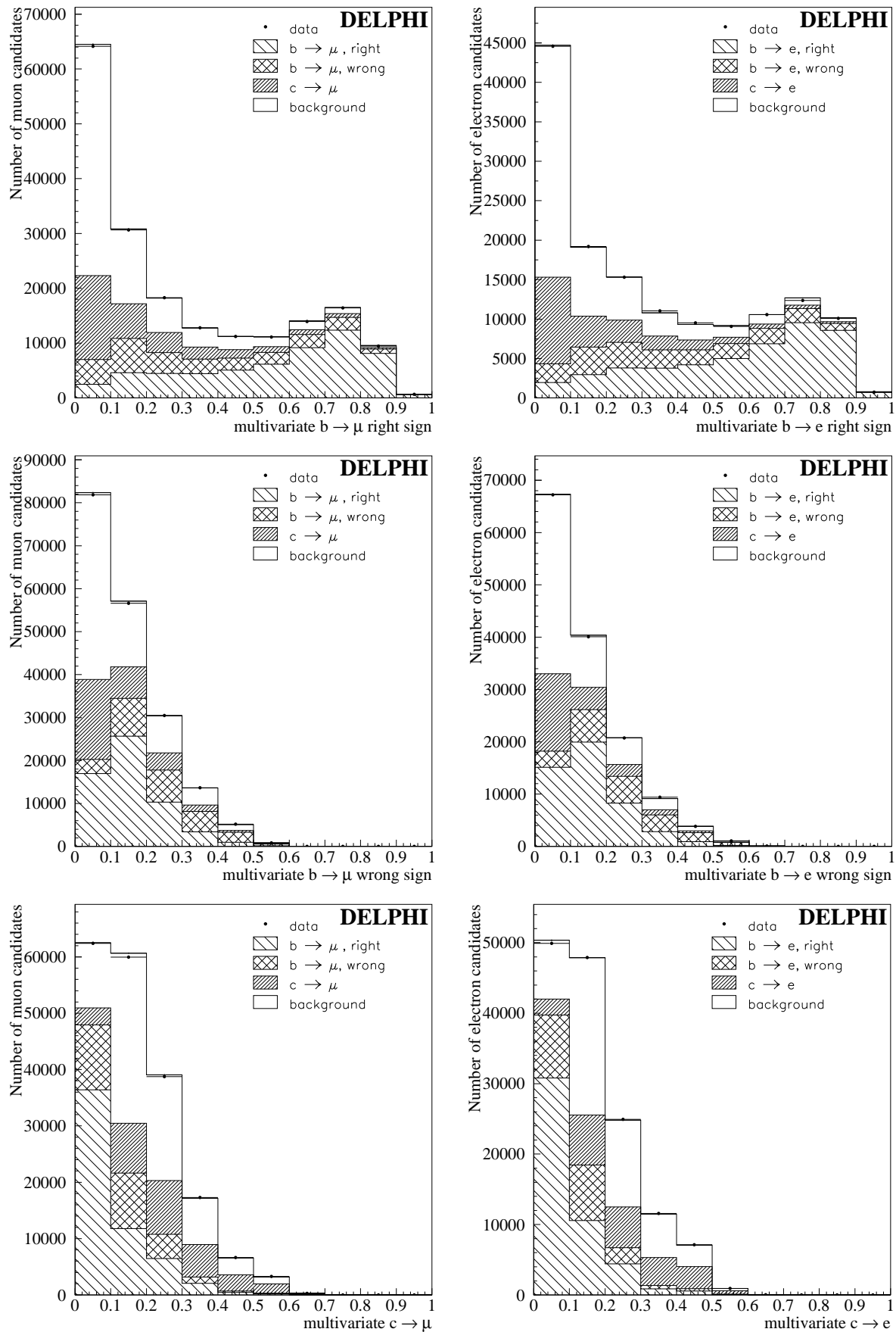
Figure 3: Likelihood ratio \mathcal{P}_{b_r} (up), \mathcal{P}_{b_w} (middle) and \mathcal{P}_c (bottom) distributions for muons (left) and electrons (right) for all years.
