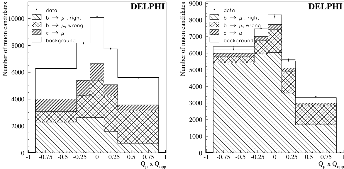
Figure 2: Jet charge distribution for the full muon sample. The muon candidates have p_T < 1.3 GeV/c and p < 7 GeV/c (left) and p_T > 1.3 GeV/c (right) corresponding to samples enriched in b \rightarrow c \rightarrow \mu^+ or b \rightarrow \mu^- events respectively.
