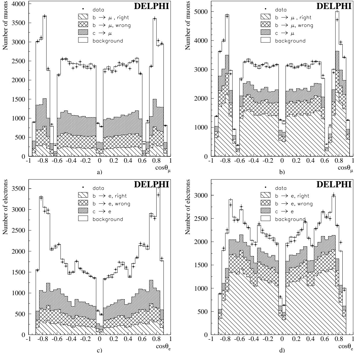
Figure 1: \cos\theta distribution for muon, upper plots, and electron, lower plots, candidates. The lepton candidates have p_T < 0.7 GeV/c in a), c) and p_T > 0.7 GeV/c in b), d) corresponding to samples enriched in background and signal respectively. The “ b \rightarrow \mu/e right (wrong)” samples correspond to leptons with the same (opposite) sign as the primary b parton (see Section 6.1). Converted photons cause the strong \cos\theta_e dependence of the background in the c) plot. Only the statistical errors are quoted in these plots. The systematics on the samples composition considered in the text are enough to cover the few discrepancies observed between the data and the simulation.
