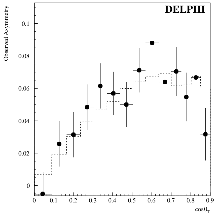
Figure 4: Observed A_{\text{FB}}^{\text{obs}} asymmetry at peak energy as a function of \cos\theta_T for a data subsample enriched in b with the right sign ( \mathcal{P}_{b_r} - \mathcal{P}_{b_w} > 0.6 ). The result of the fit is shown as a dashed line.
