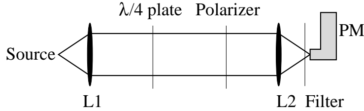
Fig. 6. Optical bench.
