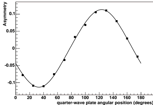
Fig. 9. Corrected asymmetry fitted by the parametrisation of equation 5.
