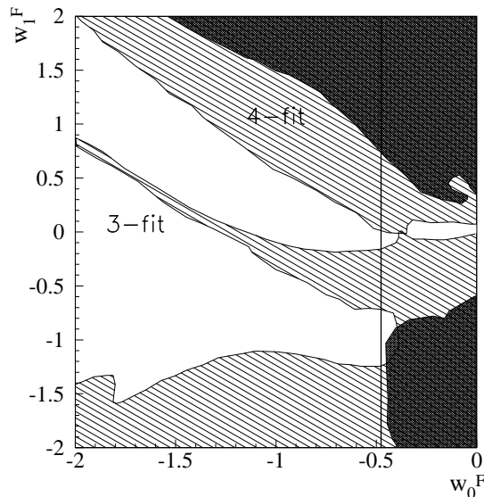
Figure 7: E(w_0, 3\text{-fit}) - \sigma(w_0, 4\text{-fit}) for the SNAP data and a weak \Omega_M prior. The white part corresponds to a positive difference, the hatched part to a negative difference, the black region corresponds to the Non Converging zones.
