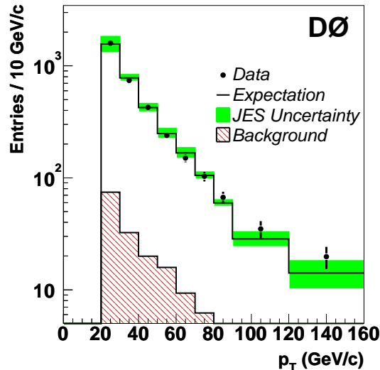
FIG. 1: The p_T distribution of taggable jets in dielectron and dimuon channels compared to Z +jet ALPGEN with PYTHIA showering and full detector simulation (open histogram), and background (multijet for ee channel and b\bar{b} background for \mu\mu channel) derived from data. The error bars on the data points are statistical. The prediction is normalized to the data, as described in the text.
