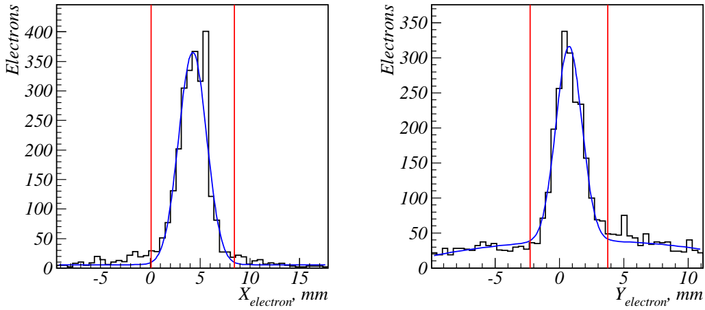
Fig. 2. The x and y coordinate of the incident electron measured by the profile monitor. Lines show the cuts used in the analysis.
