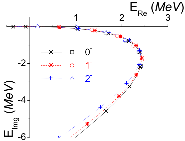
FIG. 2: Negative parity tetra-neutron resonance trajectories parametrized by the strength W of the phenomenological 4NF. ACCC results are denoted by lines with overimposed x , * , + symbols. They correspond to W values by steps of 4 \text{ MeV}\cdot\text{fm}^{-1} starting from 38 \text{ MeV}\cdot\text{fm}^{-1} for J^\pi = 0^- and 2^- states and from 36 \text{ MeV}\cdot\text{fm}^{-1} for 1^- . CS results are represented by circles, squares and triangles.
