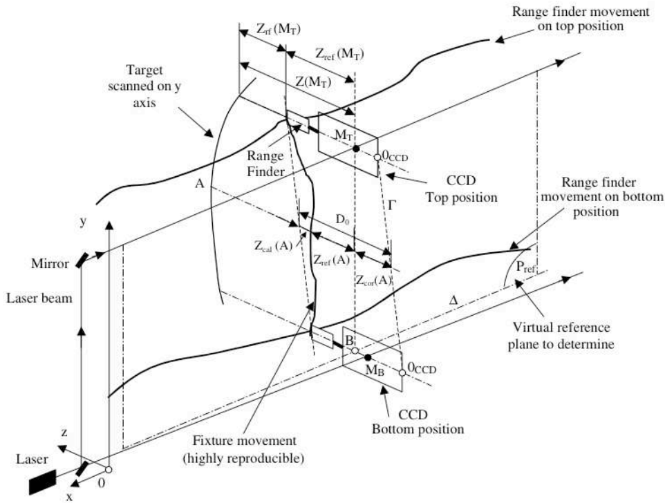
Figure 3. Geometrical description of the set-up.
