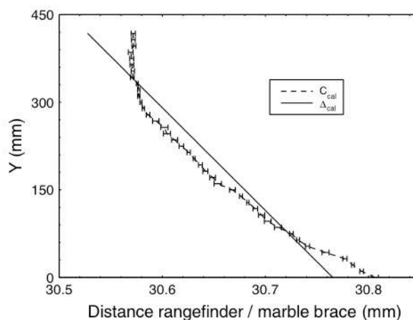
Figure 2. Y-axis calibration curve.
