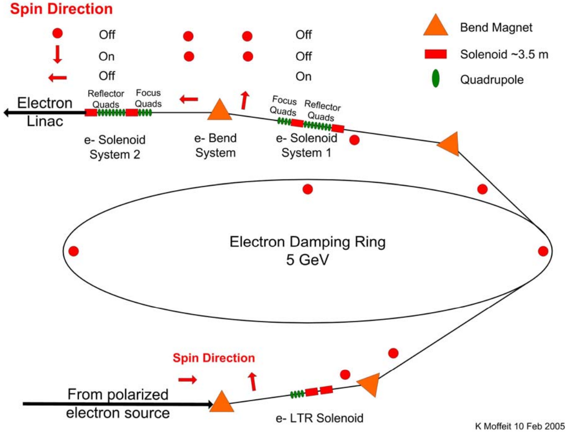
Figure 2: Layout of electron damping ring system showing the spin rotation solenoids.
