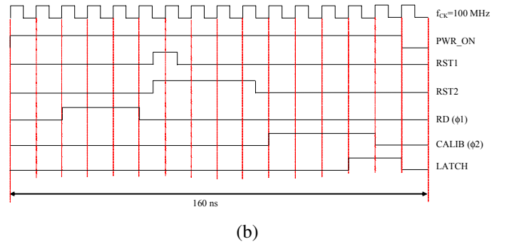
Fig. 1. (a) Schematic of the proposed DC-coupled pixel and, (b) related timing (clocking stimuli) with f_{CK} = 100 \text{ MHz} . RD, CALIB and LATCH signals are used by the column readout circuitry.
