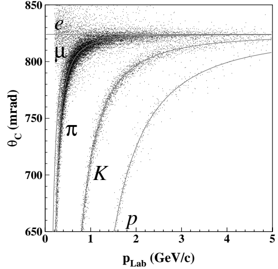
Figure 51. The fitted Cherenkov angle of tracks from an inclusive sample of multi-hadron events plotted against the momentum of the tracks at the entrance to the DIRC bar box. The grey lines are the predicted values of the \theta_C for the different particle species.
