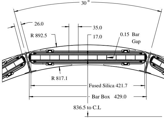
Figure 11. Cross section through the Central Support Tube showing a bulkhead, the slot liner and a bar box. The inner and outer skins are not shown. All dimensions are in millimeters.
