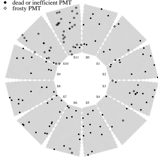
Figure 50. Location of frosty PMTs and dead or inefficient electronics channels.
