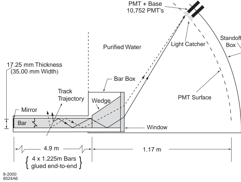
Figure 3. Schematic of the DIRC fused silica radiator bar and imaging region.
