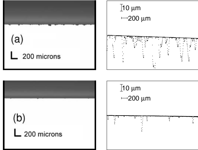
Figure 23. Example of (a) bad bar edge, as it appears on the computer screen used for the microscope readout (left side), and the digitized version of the same edge displayed by the off-line software analysis (right side), and (b) the same for the good bar edge, which was typical. The digitized plots have been greatly magnified in the y-direction.
