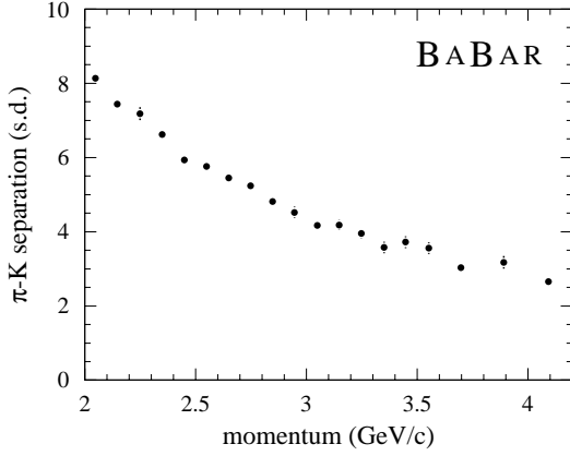
Figure 54. DIRC \pi -K separation versus track momentum measured in D^0 \rightarrow K^- \pi^+ decays selected kinematically from inclusive D^* production.
