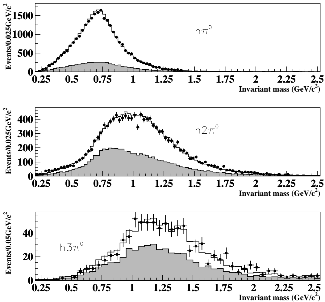
Figure 17: Invariant-mass distributions for the one-prong decays selected with the neural network. Data are shown as dots, simulation by a solid line. The shaded area shows the background prediction from simulation.
