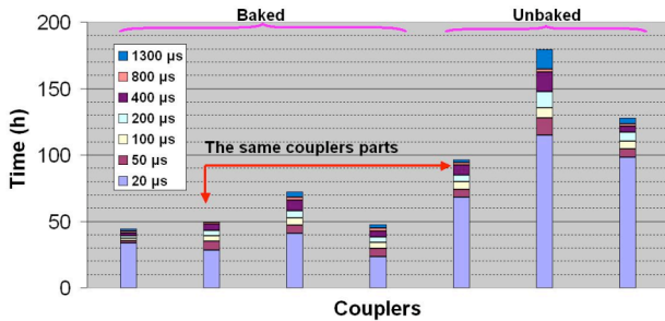
Figure 6: Conditioning time summary of seven in-situ and non in-situ baked coupler pairs.
