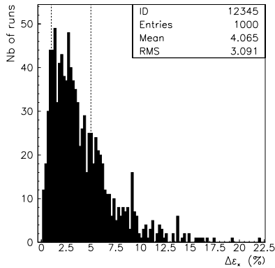
Figure 2: horizontal emittance increase when all linac quadrupoles are randomly shifted along x within \pm 0.1 \text{ mm} .
