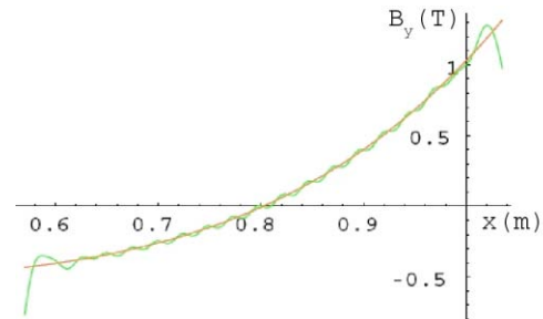
Figure 5: Comparison between theoretical field and calculated field for 20 conductors on a pole. Oscillations disappear with 80 conductors, except on extremities.
