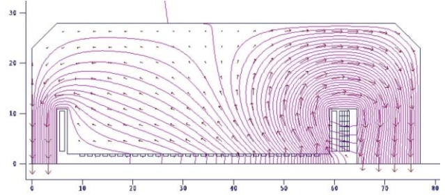
Figure 2: Poisson-Superfish simulation with parameters of spiral dipoles from the ADSR KURRI project in Japan [1].
