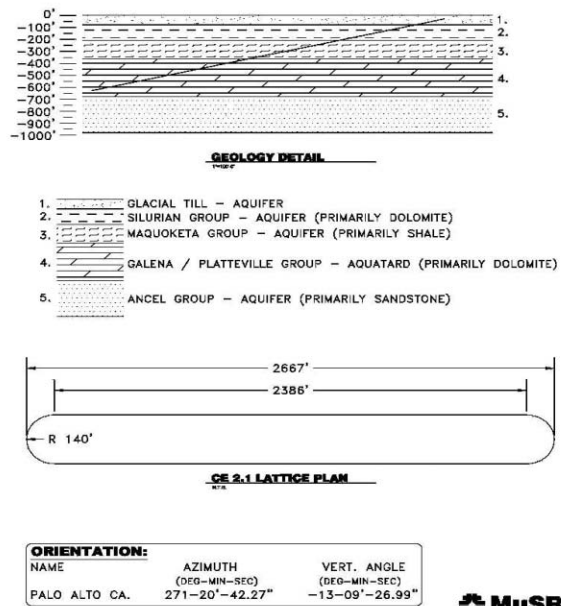
Figure 2. Constraints on the storage ring due to the geology under the Fermilab site The 2667' (or 813 meter) limit on the cross-section profile of the ring shown in the lower drawing is given by the 600 foot available for the ring's vertical drop the and 13^\circ between Fermilab and the West Coast.
