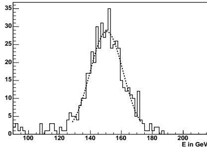
FIGURE 5. Response to 180 GeV pions that do not start showering before reaching TileCal.
