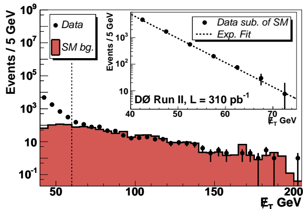
FIG. 1: Distribution in E_T after applying all criteria, except E_T > 60 GeV ( C1 ). The dark shaded area corresponds to the SM simulation. A fit by an exponential to E_T < 60 GeV, after subtraction of the contributions from the SM, shown in the figure insert, is used to estimate the instrumental background.
