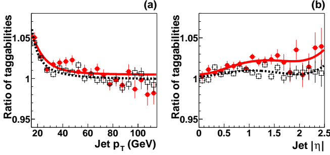
FIG. 4: Ratio of the b to light (full circles) and c to light (open squares) quark jet taggability, measured in a QCD MC sample as functions of (a) jet p_T and (b) jet |\eta| . The resulting fits used in the analysis are also shown.
