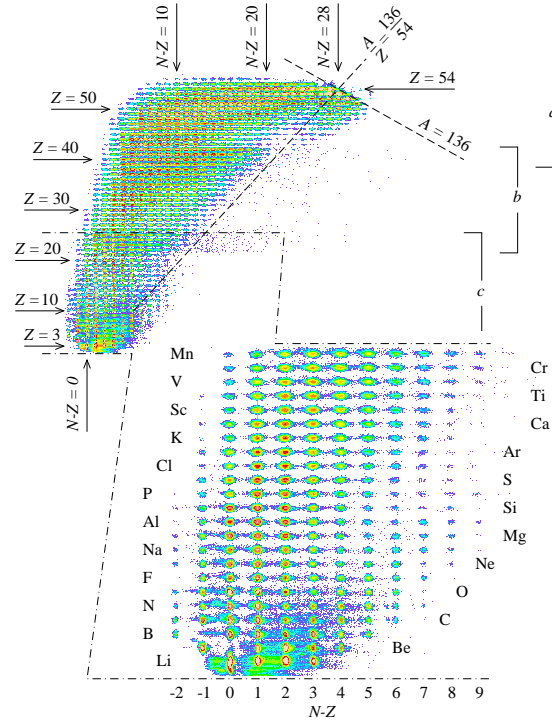
Fig. 6. Composition of all identified events measured with the FRS spectrometer with a ^{136}\text{Xe} beam at 1 A GeV on a hydrogen target. Three overlapping bands a, b, c correspond to the three groups of magnetic settings for the central isotopes ^{120}\text{Ag} , ^{69}\text{Zn} and ^{24}\text{Al} respectively. The band c collecting light nuclides is enlarged in order to show the isotopic resolution (P. Napolitani, Ph.D. thesis, University Paris XI, 2004).
