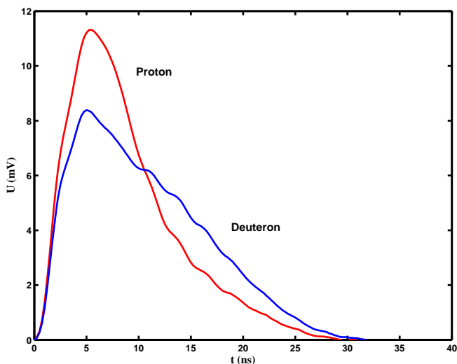
Fig. 8. Example of a mean experimental current signal sampling for two kind of particles, proton and deuteron, at the same incident energy 5 MeV [39].
