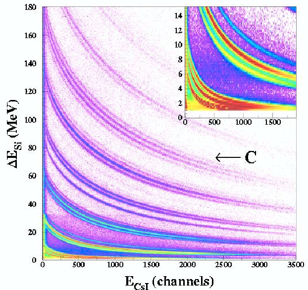
Fig. 4. An example of a \Delta E - E matrix for the Lassa-Hira setup.
