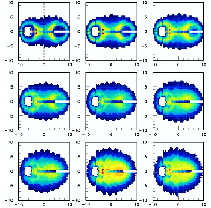
Fig. 2. Alpha particles centre-of-mass v_{\text{parallel}}-v_{\text{perpendicular}} plots for different dissipation regimes measured with the INDRA multidetector in Xe+Sn collisions at 80 A MeV. Peripheral to central collisions are displayed from upper-left to bottom-right panel (M.Pichon, PhD. Thesis, Caen University 2003).
