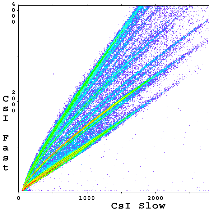
Fig. 1. Fast-Slow INDRA CsI matrix obtained by accumulating high-energy light charged particles coming from two reactions, ^{124}\text{Xe}+^{112}\text{Sn} and ^{136}\text{Xe}+^{124}\text{Sn} at 45 A MeV, during the fifth INDRA campaign at Ganil. Isotopic identification is obtained for H, He, Li, Be and B produced during the collisions.
