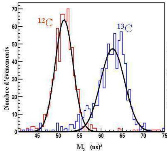
Fig. 10. Discrimination of carbon isotopes. Histograms correspond to the distributions of the second moment values M_2 of pulses and full line to Gaussian fits see [39].
