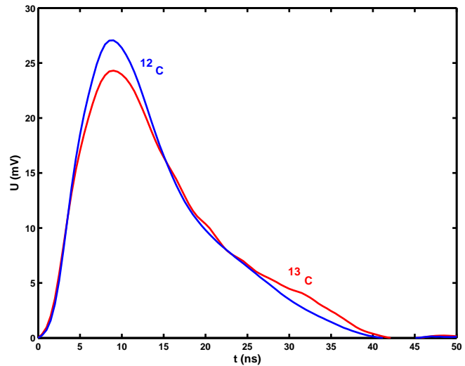
Fig. 9. Example of a mean experimental current signal sampling for two carbon isotopes, ^{12}\text{C} and ^{13}\text{C} , at the same incident energy 80 MeV. Isotopic determination is well established with the second moment values M_2 of digitized current pulse, see [39] and figure 10.
