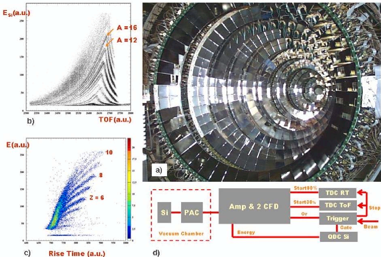
Fig. 3. a) Forward part of the CHIMERA detector (as seen by the target). b) Plot Energy from silicon detector - Time of Flight for reaction products of Ne+Al at 20 A MeV (detected at \theta=12^\circ and at 180 cm from the target). Charged particles stopped (low kinetic energy) in the first stage silicon detector or (alternatively) stopped in the second stage CsI(Tl) crystal are seen in the plot. c) Plot Energy - Signal Rise Time showing the charge identification obtained with the PSD only for charged particles that are stopped in the Silicon detector. d) Electronic chain of CHIMERA as upgraded for the PSD analysis with silicon detector.
