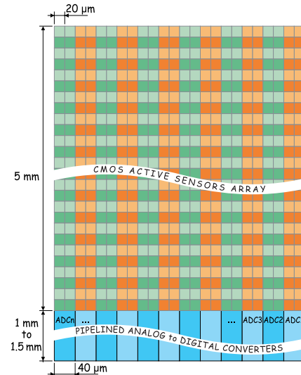
Figure 1: Sketch view of a MAPS array with a data conversion stage.
