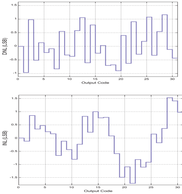
Figure 12: Non linearity results.
