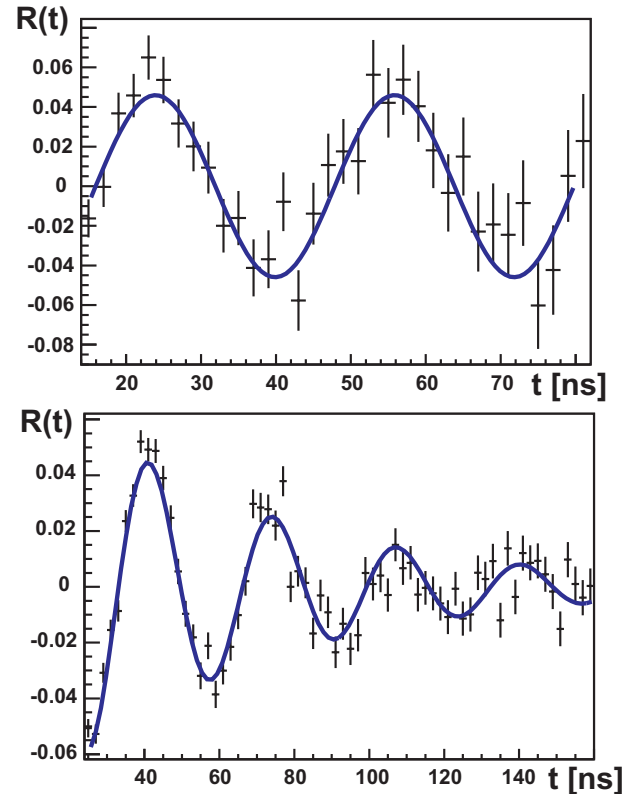
Fig. 2. R(t) functions for the "all together" combination of the Ge (upper part) and BaF 2 (lower part) detectors. See the text for more details.
