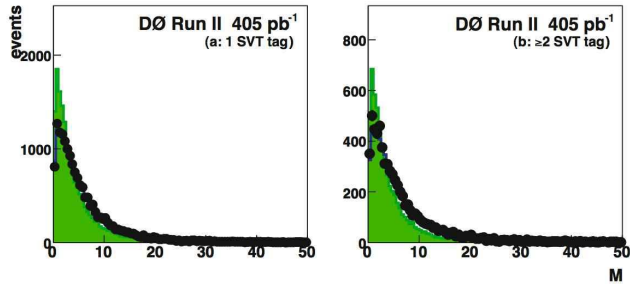
FIG. 5: The \mathcal{M} distribution for single-tag events (a) and double-tag events (b). Shown are the data (points), the background (solid line) and the expected t\bar{t} distribution (filled histogram) multiplied by 140 (60) for the single (double)-tag analysis.
