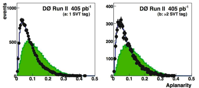
FIG. 3: The \mathcal{A} distribution for single-tag events (a) and double-tag events (b). Shown are the data (points), the background (solid line) and the expected t\bar{t} distribution (filled histogram) multiplied by 140 (60) for the single (double)-tag analysis.
