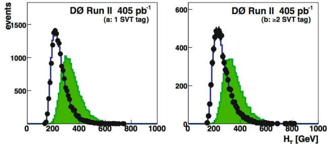
FIG. 1: The H_T distribution for single-tag events (a) and double-tag events (b). Shown are the data (points), the background (solid line) and the expected t\bar{t} distribution (filled histogram) multiplied by 140 (60) for the single (double)-tag analysis.
