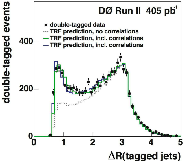
FIG. 8: The performance of the TRF prediction on double-tag events (points), without including the correlation factor C_{ij} (dashed histogram), and including C_{ij} for two different functional parameterizations (solid histograms).
