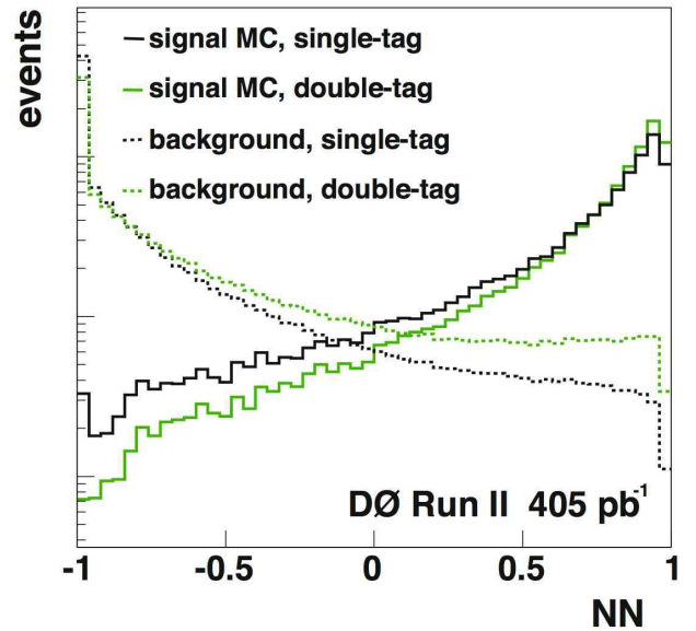
FIG. 7: The output discriminant of an artificial neural network ( NN ) with six input nodes. All distributions are normalized to area. NN is optimized to distinguish between fully hadronic t\bar{t} Monte Carlo events (signal) and the background from multijet production (background) as predicted by the tag rate functions.
