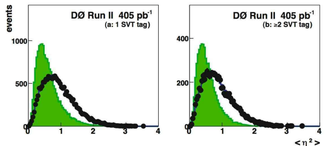
FIG. 4: The \langle \eta^2 \rangle distribution for single-tag events (a) and double-tag events (b). Shown are the data (points), the background (solid line) and the expected t\bar{t} distribution (filled histogram) multiplied by 140 (60) for the single (double)-tag analysis.
