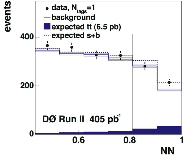
FIG. 9: The distribution of the NN output variable for single-tag events. Shown are the data (points), background (hashed band), signal (filled histogram) and signal+background (dashed histogram). The vertical line represents the used cut of NN > 0.81 .
