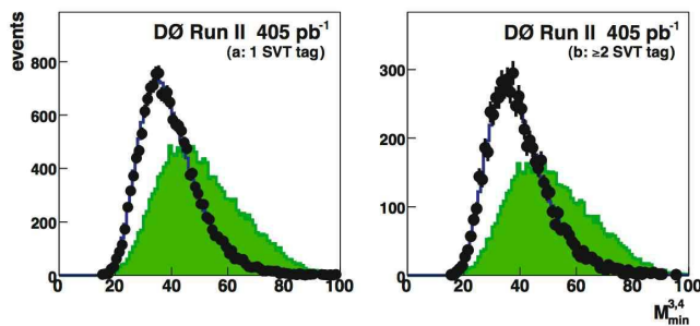
FIG. 6: The M_{min}^{34} distribution for single-tag events (a) and double-tag events (b). Shown are the data (points), the background (solid line) and the expected t\bar{t} distribution (filled histogram) multiplied by 140 (60) for the single (double)-tag analysis.
