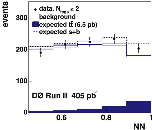
FIG. 10: The distribution of the NN output variable for double-tag events. Shown are the data (points), background (hashed band), signal (filled histogram) and signal+background (dashed histogram). The vertical line represents the used cut of NN > 0.78 .
