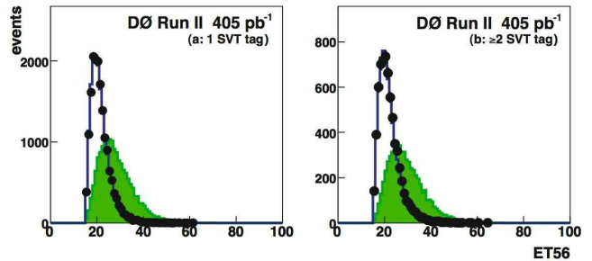
FIG. 2: The E_T^{56} distribution for single-tag events (a) and double-tag events (b). Shown are the data (points), the background (solid line) and the expected t\bar{t} distribution (filled histogram) multiplied by 140 (60) for the single (double)-tag analysis.
