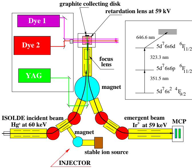
Fig. 2. The COMPLIS setup. The insert shows the ionization scheme used in this experiment.
