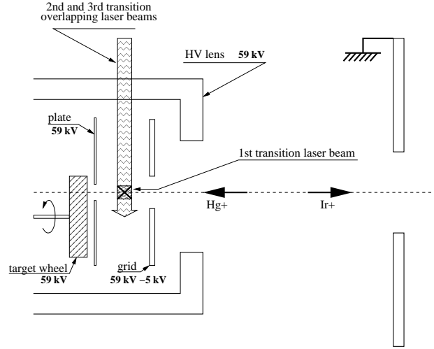
Fig. 3. Schematic view of the interaction chamber of the COMPLIS setup. The graphite substrate is located on a rotating target wheel. The first step laser beam is in the horizontal direction while the second and third transition laser beams are in the vertical direction.
