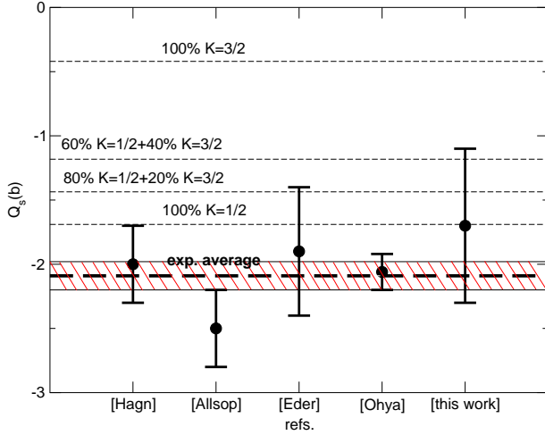
Fig. 19. Experimental Q_s values for ^{185}\text{Ir} available in the literature: from Static nuclear Orientation with \gamma detection: Hagn et al. [43] and Allsop et al. [44] and from Nuclear Magnetic Resonance on Oriented Nuclei: Eder et al. [80] and Ohya et al. [35]. A thick dashed line indicates the weighted average of the experimental values and the hatched zone represents the probable error of the mean. The others thin dashed lines correspond to different K mixing situations.
