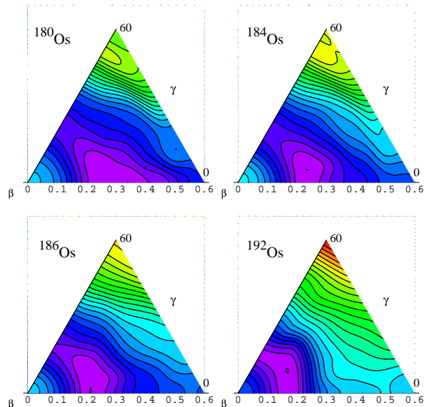
Fig. 15. Potential energy surface V(\beta, \gamma) calculated for ^{180,184,186,192}\text{Os} obtained in the constrained HFB calculations [72]. Contours are separated by 1 MeV.
