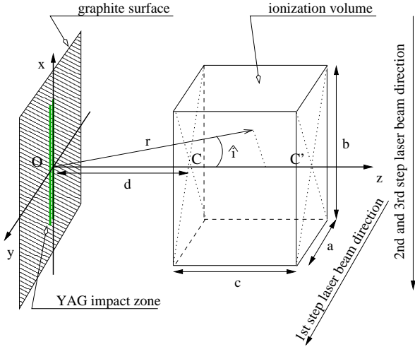
Fig. 9. Geometry of the ionization process: the ionization volume defined by the three laser beam spatial overlap is assumed to be a parallelepiped of sides (a, b, c) .
