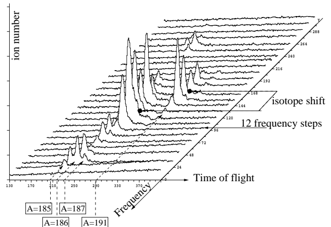
Fig. 5. An example of a data matrix of ion numbers as a function of time of flight and frequency obtained during this experiment. Each time of flight curve which is represented here is actually a sum of 12 recorded time of flight curves i.e. 12 frequency steps.
