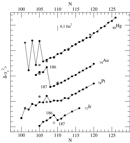
Fig. 14. Mean square charge radius variation obtained from the IS measurement for different isotopic series in the Pt region. Isomeric states are represented by open circles.
