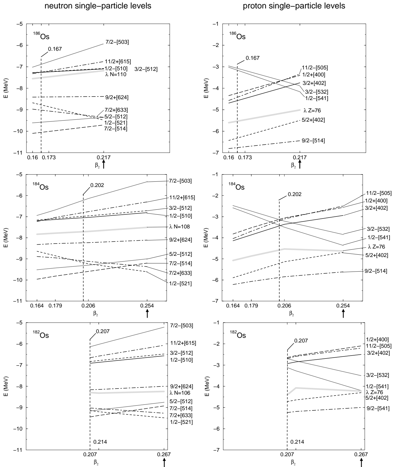
Fig. 16. Energies of the neutron and proton sp-states in the HF field of the even-even cores ^{186}\text{Os} ( N=110 ), ^{184}\text{Os} ( N=108 ) and ^{182}\text{Os} ( N=106 ) as a function of the axial deformation parameter. The Fermi levels are indicated with thick grey lines. The values of the axial deformation parameter at which the calculations were performed are indicated on the horizontal axis. The deformation values obtained for equilibrium (constraint free calculations) are indicated by arrows, those of the odd Ir nuclei deduced from the IS measurements are indicated by vertical dotted lines.
