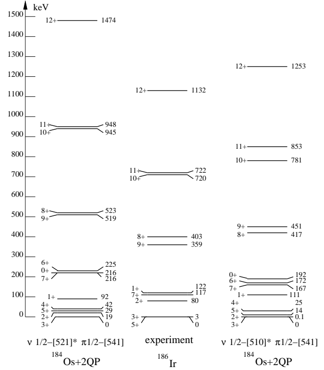
Fig. 20. The two calculated bands built on the \nu 1/2^- [521] \otimes \pi 1/2^- [541] and the \nu 1/2^- [510] \otimes \pi 1/2^- [541] main configurations compared with the experimental ^{186}\text{Ir} ground state band. A ^{184}\text{Os} core at \beta_2 = +0.206 was used.
