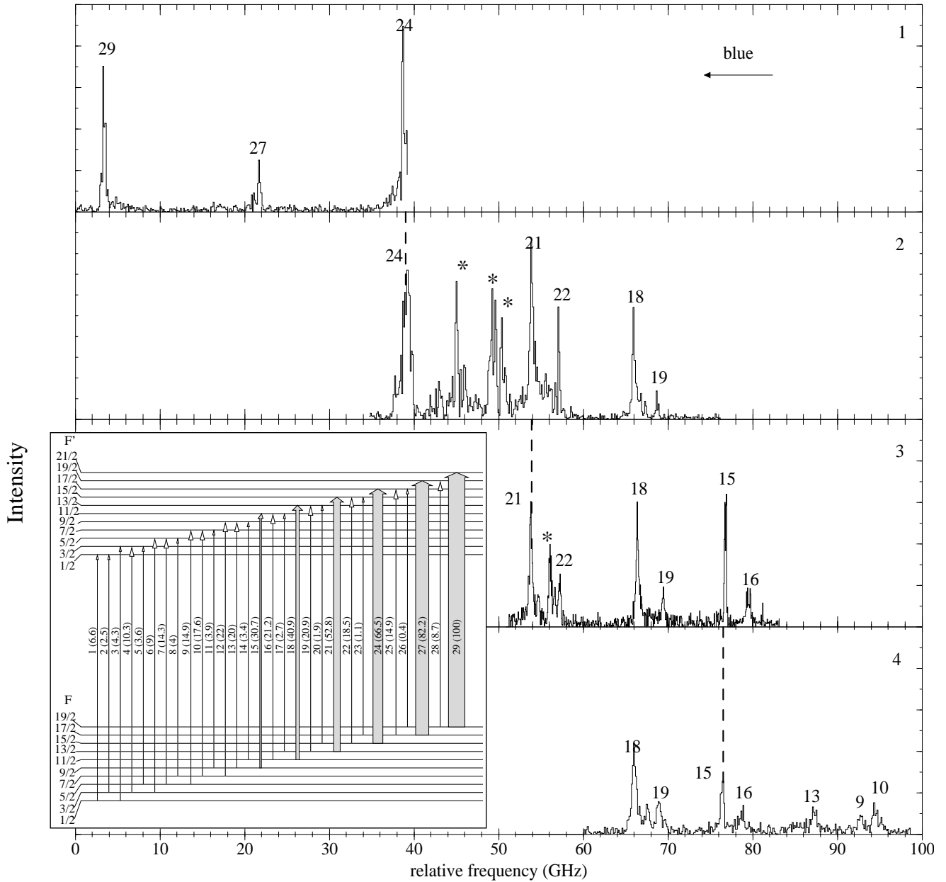
Fig. 12. Partial recordings of the hyperfine spectra of ^{186}\text{Ir}^g and ^{186}\text{Ir}^m . The common peaks used in order to link the different parts are indicated by dotted lines. Each peak is identified by the labels of the hyperfine transitions displayed in the insert (the relative intensities are indicated between parentheses). Peaks belonging to the isomeric state are indicated with *-symbols.
