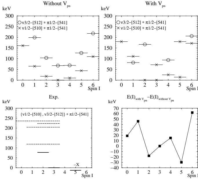
Fig. 21. Upper part: first levels with their main component on \nu 1/2^- [510] \otimes \pi 1/2^- [541] and on \nu 3/2^- [512] \otimes \pi 1/2^- [541] calculated with a ^{184}\text{Os} core with a constraint of \beta_2 = 0.206 with and without including the residual proton-neutron interaction. Lower part: experimental levels from [92]. When the spin assignment is uncertain, the levels are represented with dashed lines covering the range of the proposed values. On lower right are represented the difference in energy between the first level of the \nu 1/2^- [510] \otimes \pi 1/2^- [541] band calculated with and without the neutron-proton interaction.
