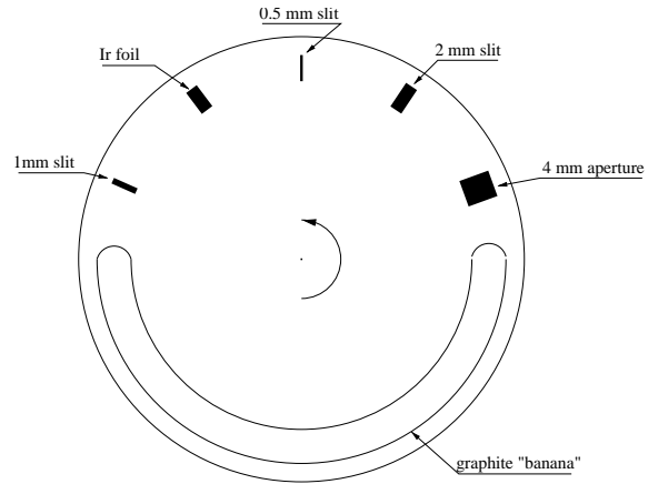
Fig. 8. Front view of the target wheel. To allow implantation - desorption on a large area, the graphite surface is shaped into a “banana”. Various target positions are left as open apertures so that a Faraday cup can be used to measure beam current passing through. Before the measurements, the incident beam line parameters are set for an optimized current in the 1 mm slit. Desorption is performed on a Ir foil for settings which need a continuous and large amount of stable Ir isotopes to be available.
