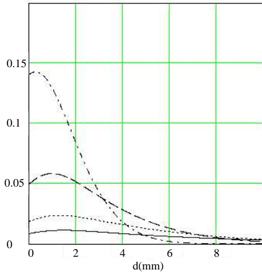
Fig. 10. Probability for one desorbed atom to be inside the ionization parallelepiped as a function of the distance d between the graphite surface and the three laser beam overlap region after a diffusion delay of t_d = 5\mu\text{s} (dot-dashed line), t_d = 10\mu\text{s} (dashed line), t_d = 15\mu\text{s} (dotted line) and t_d = 20\mu\text{s} (solid line).
