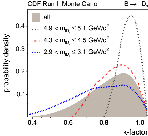
Figure 2. k -factor distribution for several m(\ell D) mass regions for B_s^0 \rightarrow D_s^- \ell^+ \nu, D_s^- \rightarrow \phi \pi^- decays.
