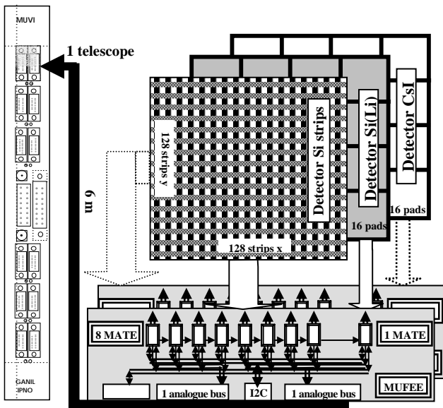
Figure 2: the electronic of one telescope
