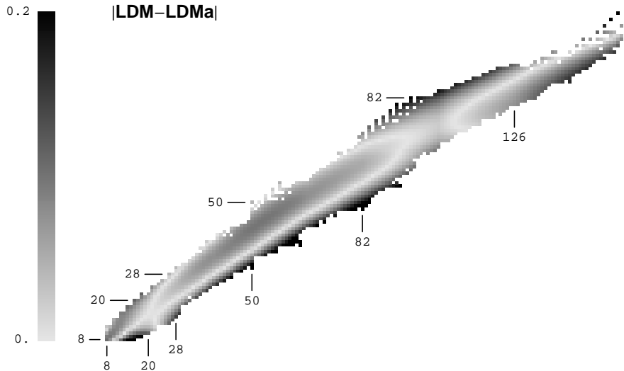
Fig. 1. Differences between calculated binding energies (in MeV) for nuclei with N, Z \geq 8 . The binding energies are calculated with the extended LDM formula (4) and with its approximation (5). In each case shell and deformation corrections have been added. The parameters in both formulas are independently adjusted to the measured binding energies of all nuclei (with N, Z \geq 8 ) in the 2003 atomic mass evaluation 11 .
