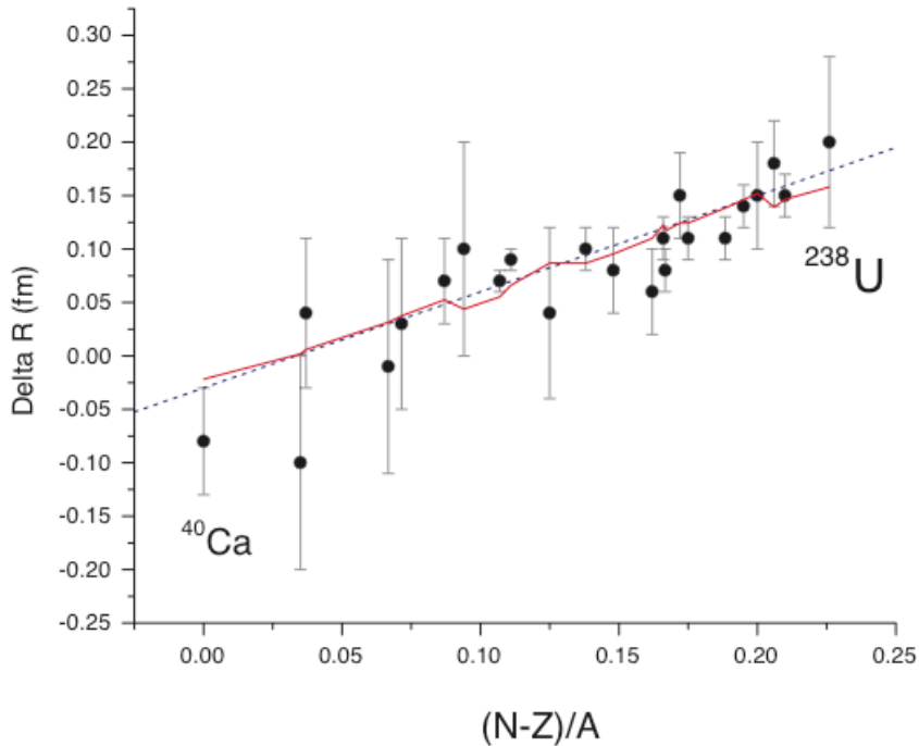
Fig. 5. The neutron-skin data \Delta R from anti-protonic atoms for nuclei between ^{40}\text{Ca} and ^{238}\text{U} . The full line is obtained from the LDM expression (6) with a volume symmetry energy S_v = 30 MeV and a volume-to-surface ratio y_s = 1.8 . The dashed line is the fit \Delta R = -0.03 + 0.90(N - Z)/A given by Schmidt et al. 28 .
