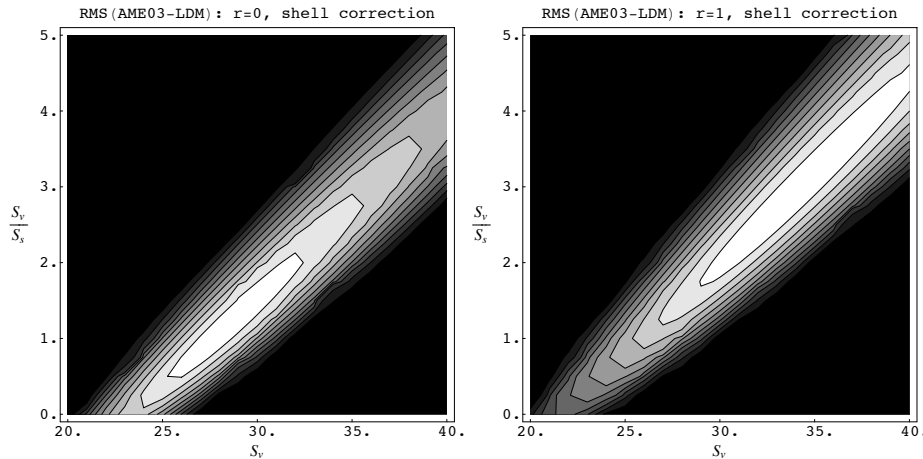
Fig. 2. Correlation plot of S_v versus y_s = S_v/S_s for r = 0 (left) and r = 1 (right). The white areas correspond to the combination of S_v and y_s giving rise to the lowest rms deviation \sigma , i.e. \sigma = 1.65 MeV for r = 0 and \sigma = 1.40 MeV for r = 1 . Each contour interval corresponds to an increase of the rms deviation by 100 keV.
