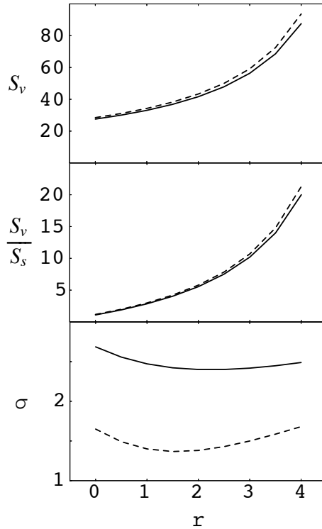
Fig. 4. The coefficient S_v (in MeV), the ratio y_s = S_v/S_s and the rms deviation \sigma (in MeV) as a function of r , obtained with the LDM formula (4) without and with shell corrections (full and dashed lines, respectively).
