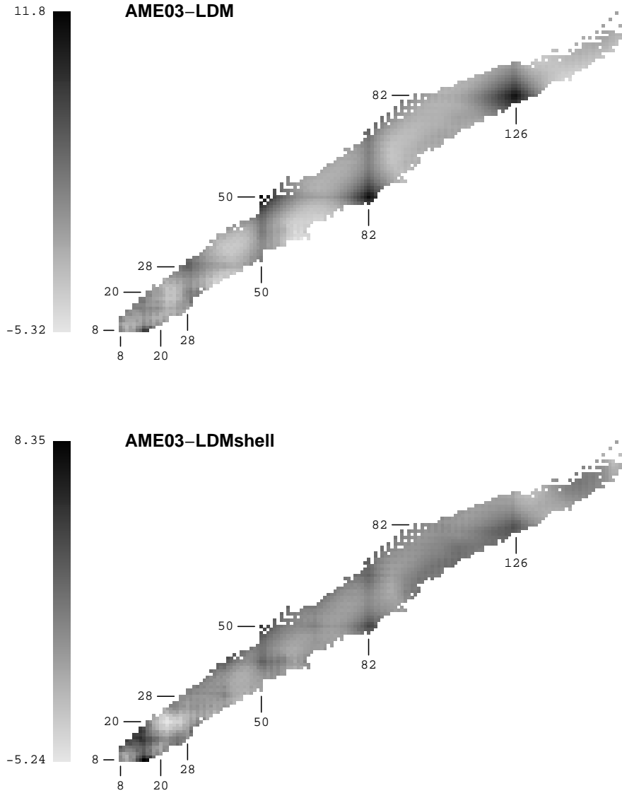
Fig. 3. Differences between measured and calculated binding energies for nuclei with N, Z \geq 8 . The binding energies are calculated with Eq. (13) which includes surface-symmetry and Wigner energies. The top figure is obtained without corrections due to shell structure while the bottom figure includes the two-parameter term (12). A colour version of the figure, showing more clearly the differences, is available on request.
