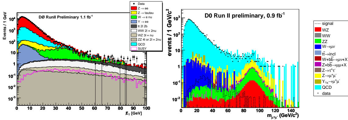
FIGURE 1. \cancel{E}_T in the ee + \ell channel (left) and invariant mass in the ls \mu\mu channel (right).
