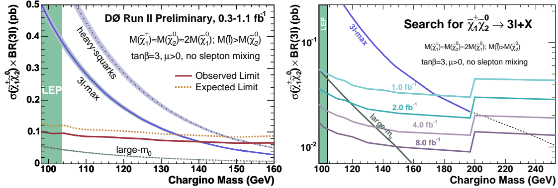
FIGURE 2. Upper limit on the \sigma \times Br(3\ell) (left) and future predictions (right) as function of m_{\tilde{\chi}_1^\pm} .
