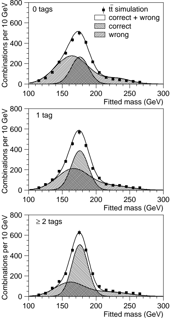
FIG. 3: Prediction of the shapes of the fitted mass distribution for the wrong and the correct permutations (hatched) and the sum of the two (black line) using the fitted parameters shown in Table III. The sum of the two is compared to the simulated data containing a weighted sum of all solutions (correct and wrong), for the default jet energy scale and a generated top quark mass of 175 GeV for events with 0 (upper), 1 (middle), or more than 1 (lower) b tags.
