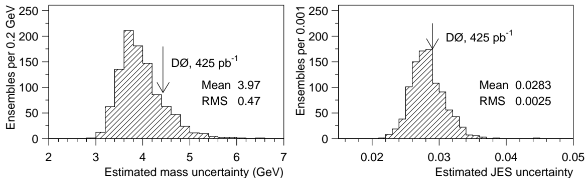
FIG. 9: Distribution of the estimated statistical uncertainty on the top quark mass measurement (left) and JES measurement (right) for the fully calibrated analysis, in the combined lepton+jets channel. The values observed in data are indicated by the arrows.
