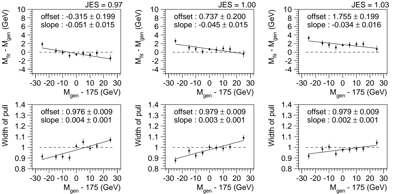
FIG. 6: The difference between the mean fitted mass M_{\text{fit}} and the generated top quark mass M_{\text{gen}} as a function of the generated top quark mass for a “true” JES of 0.97 (left), 1.00 (middle), and 1.03 (right), for the lepton+jets channel ( e + \mu combined). At a generated mass of 175 GeV, the mass bias changes by 1 GeV when the true JES is varied by \pm 3\% .
