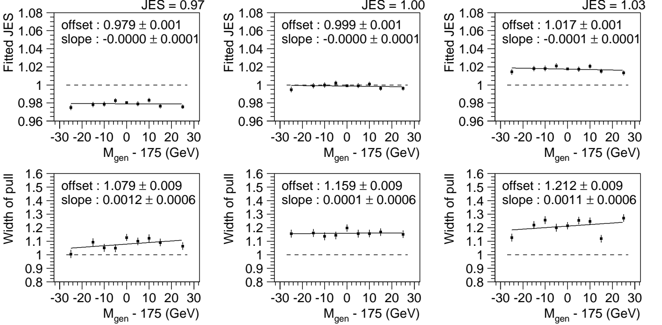
FIG. 5: The mean fitted JES and pull width as a function of the generated top quark mass M_{\text{gen}} for a “true” JES of 0.97 (left), 1.00 (middle), and 1.03 (right), for the lepton+jets channel ( e + \mu combined). The fitted JES is stable as a function of generated top quark mass.
