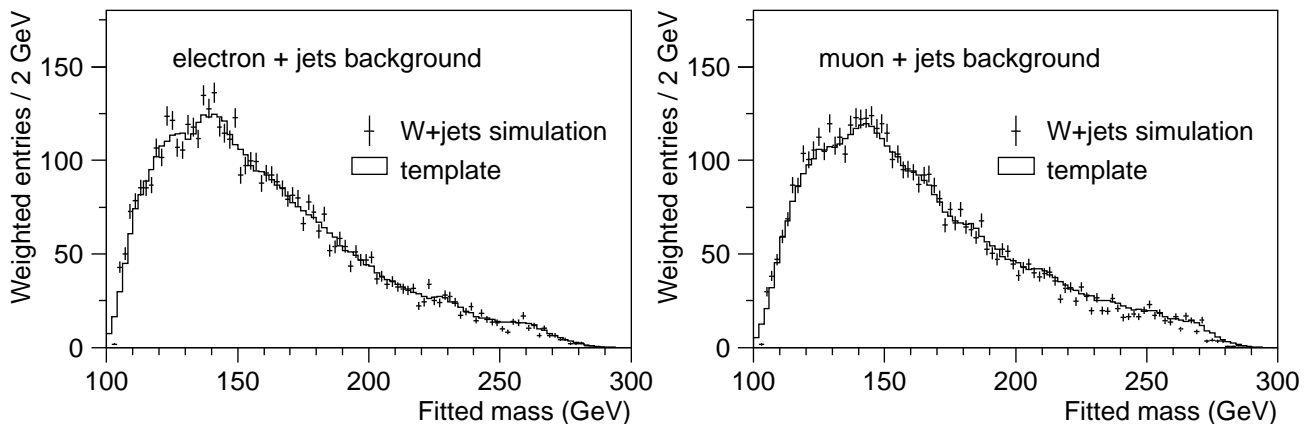
FIG. 2: Histograms showing the background shape from a weighted sum (see text) of all twenty-four masses from each event from the W +jets background sample (points with error bars), for the electron+jets channel (left) and muon+jets (right). The histograms show the shapes that are used in the likelihood. To reduce statistical fluctuations, the shapes are calculated as the average value in a sliding window of \pm 5 GeV around each fitted mass.
