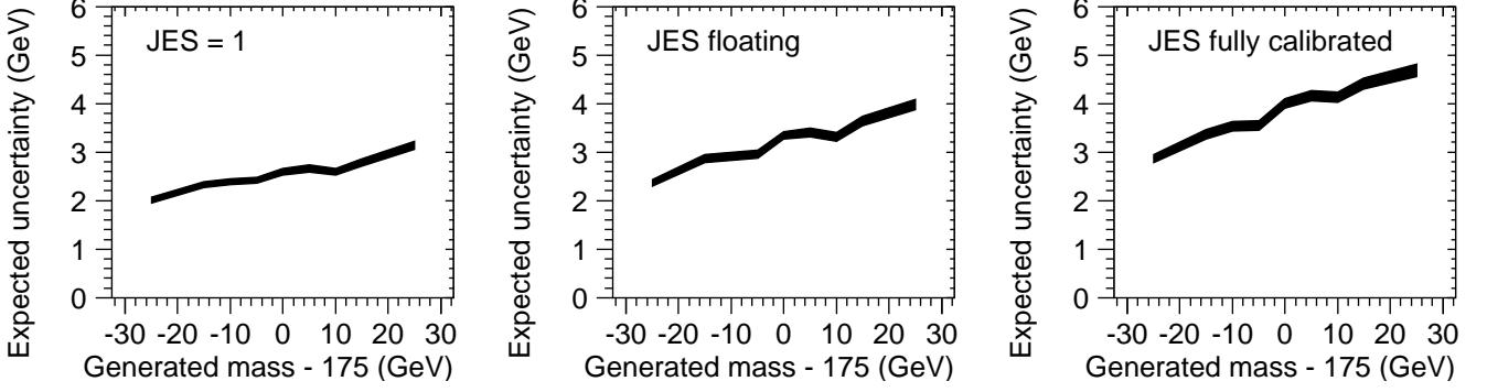
FIG. 7: The expected statistical uncertainty from ensemble tests is shown as a function of the generated top quark mass for three scenarios: with the JES parameter fixed to 1 (left), allowing the JES parameter to float freely in the fit, but only calibrating the mass fit for a true JES = 1 (middle), allowing the JES parameter to float freely in the fit and applying the full calibration as a function of true top quark mass and true JES (right). In each plot the width of the band indicates the estimated uncertainty.
