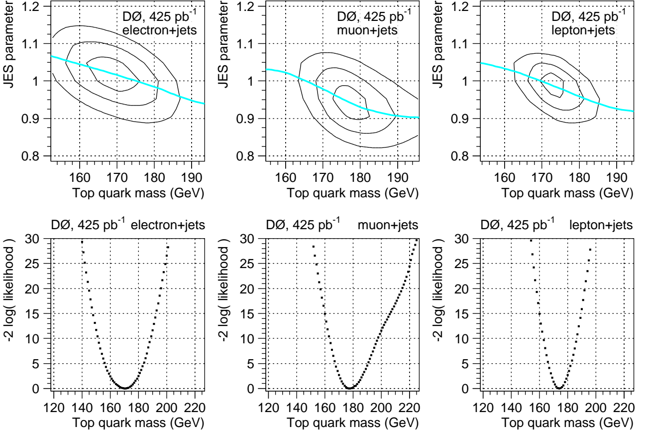
FIG. 8: Overall likelihood curves for the events observed in data, in the electron+jets channel (left), muon+jets (middle), and both channels combined (right). The top plots show the full 2-dimensional likelihood as a function of the jet energy scale parameter ( JES ) and top quark mass. Each contour, n , corresponds to a difference in likelihood of \Delta \ln(\mathcal{L}) = -n^2/2 with respect to the maximum likelihood. The fitted value of the JES parameter as a function of the top quark mass is plotted as the gray line superimposed on the 2D likelihoods. The bottom plots show the likelihood as a function of the top quark mass along the gray line from the upper plots. The fitted values from these distributions have to be corrected for the calibration from MC simulation to obtain the final results.
