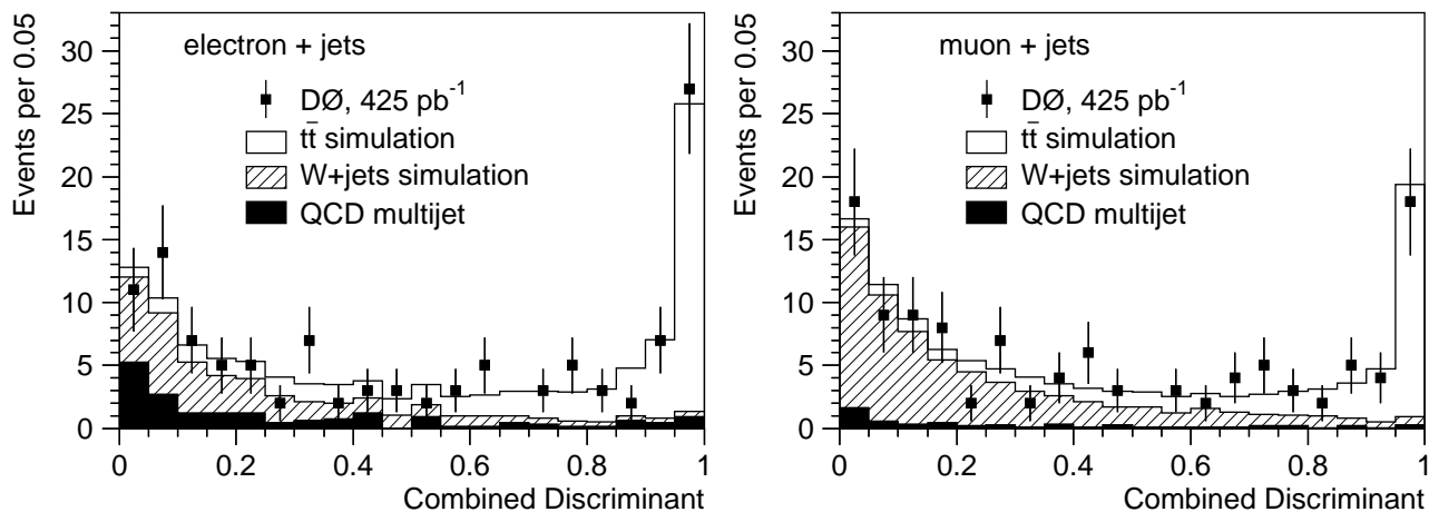
FIG. 1: Combined likelihood discriminant D in data and MC simulation in the electron+jets channel (left) and muon+jets channel (right). The t\bar{t} , W +jets and multijet contributions are normalized according to the fitted fractions.
