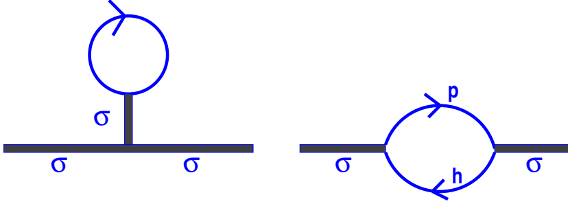
Fig. 1. Sigma self-energy in the nuclear medium.
