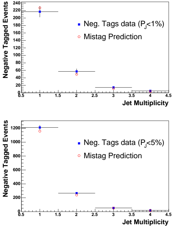
FIG. 17: Events with negative tagged jets compared to the prediction using the mistag matrix. We select events in the high- p_T lepton sample with \cancel{E}_T < 20 GeV. P_J cuts of 1% and 5% are used on the top and bottom plots respectively.
