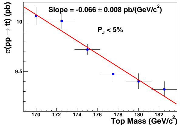
FIG. 20: Top pair production cross sections as a function of the top quark mass for P_J < 1\% (top) and P_J < 5\% (bottom). The uncertainties shown are the statistical uncertainties on the acceptances for each mass.
