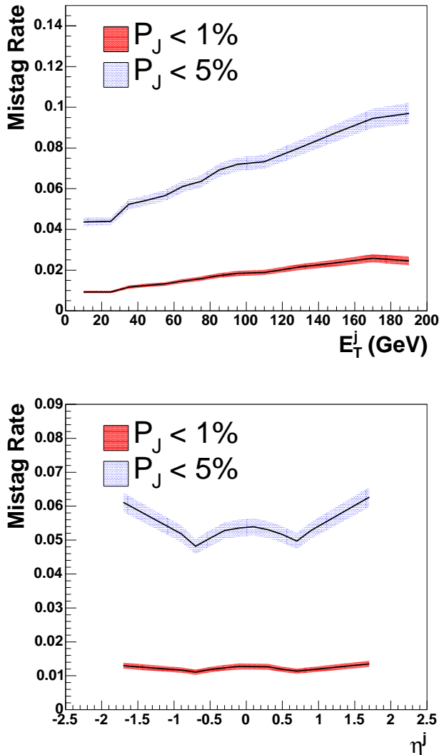
FIG. 7: Mistag rate for jet probability cuts of 1% and 5% as a function of jet E_T (top) and jet pseudo-rapidity (bottom) in inclusive jet data sample. The bands represent the statistical and systematic uncertainties added in quadrature.
