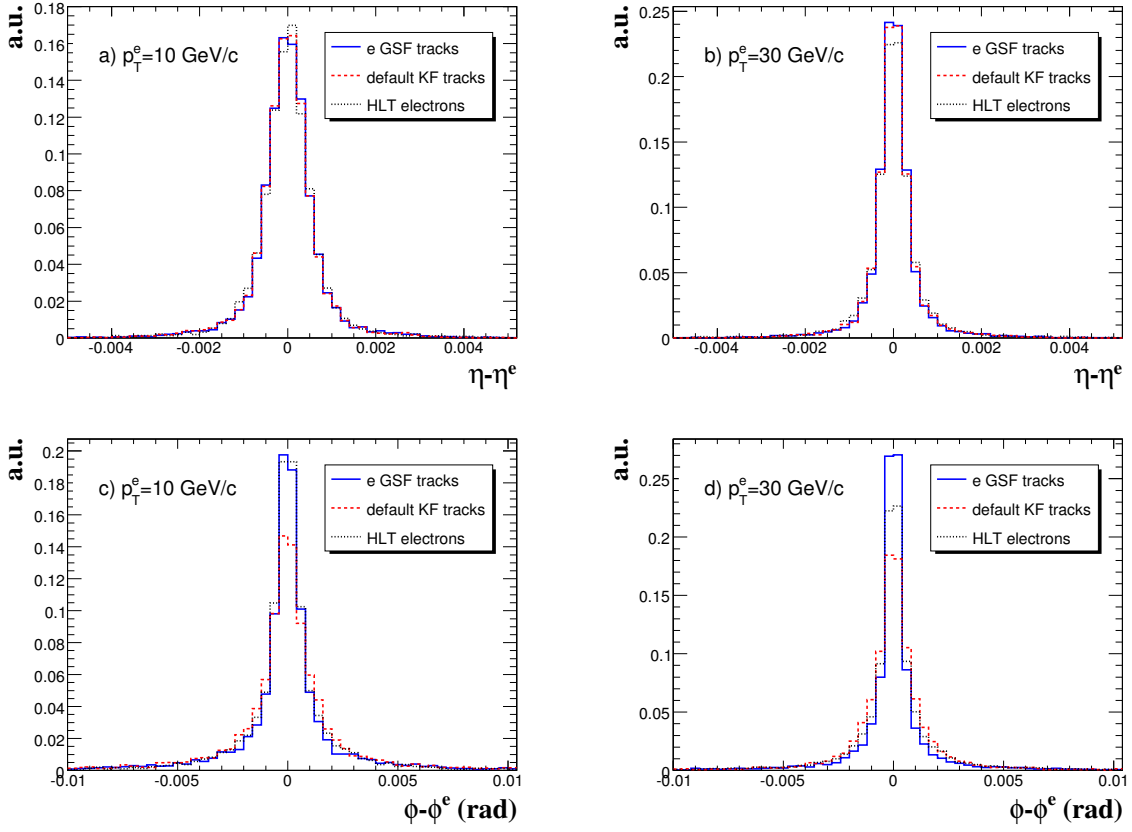
Figure 6: Difference between the reconstructed track direction at vertex and the generated one: a) \eta direction and c) \phi direction for p_T^e = 10 GeV/c electrons; b) \eta direction and d) \phi direction for p_T^e = 30 GeV/c electrons. Distributions are shown for Gaussian Sum Filter tracks (full histogram), Kalman Filter tracks (dashed histogram) and HLT electron tracks (dash-dotted histogram).
