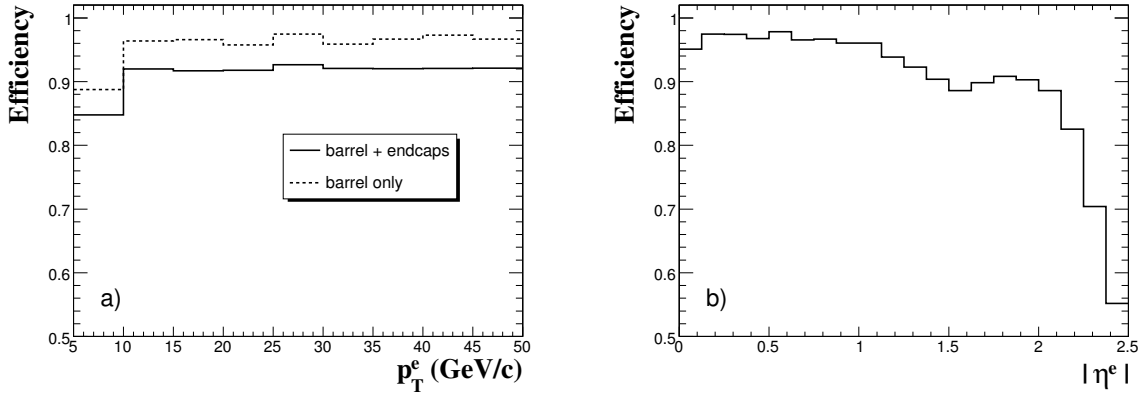
Figure 3: Electron track reconstruction efficiency (a) as a function of p_T and (b) as a function of |\eta| , for electrons uniformly distributed in p_T between 5 and 50 \text{GeV}/c . In (a), the efficiency is shown averaged over \eta the full ECAL barrel and endcaps \eta range (full line) and for the barrel only (dotted line).
