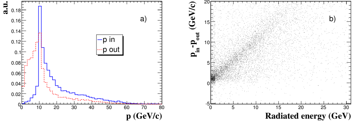
Figure 10: Estimation of the bremsstrahlung radiated energy using the GSF track parameters, for electrons with p_T^e = 10 \text{ GeV}/c ; a) track momentum evaluated at the vertex (full histogram) and at the outermost hit (dashed-dotted histogram); b) difference between track momentum at vertex and at outermost state against the energy radiated via bremsstrahlung photons along the electron trajectory. The momentum is obtained from the weighted mean of the Gaussian mixture.
