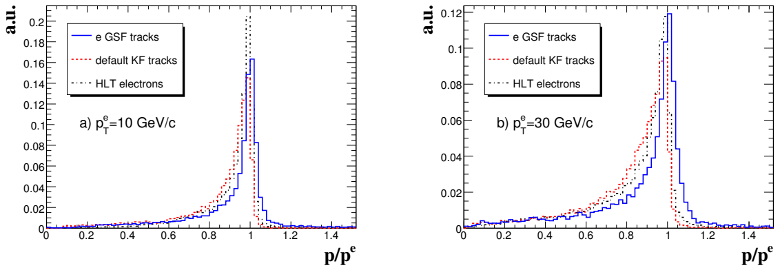
Figure 7: Ratio between the reconstructed momentum at vertex and the generated one for (a) p_T^e = 10 GeV/c electrons and (b) p_T^e = 30 GeV/c electrons. Distributions are shown for Gaussian Sum Filter tracks (full histogram), Kalman Filter tracks (dashed histogram) and HLT electron tracks (dash-dotted histogram).
