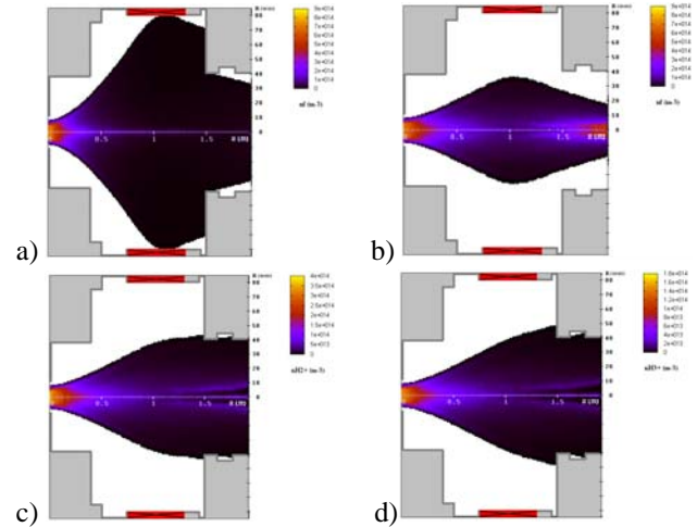
Figure 11: Distribution for the protons at 1\mu s in a), at 6\mu s in b), for the H_2^+ in c) and the H_3^+ in d) at the equilibrium.
