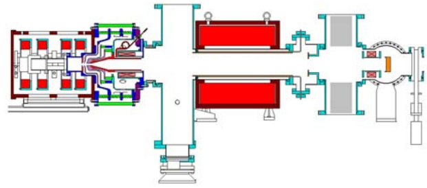
Figure 10: Schematic view of the simulated part of the LEBT.
