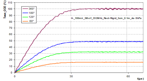
Figure 6: Evolution of the neutralization for a H^+ bunched beam for different bunch length (0.1 A, 95keV, 4.10^{-5} hPa).
