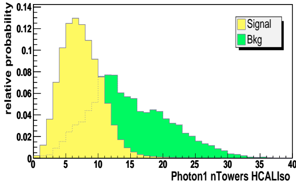
Figure 5: Number of HCAL towers hit within a cone \Delta R < 0.3 around the highest E_T photon at the preselection level.
