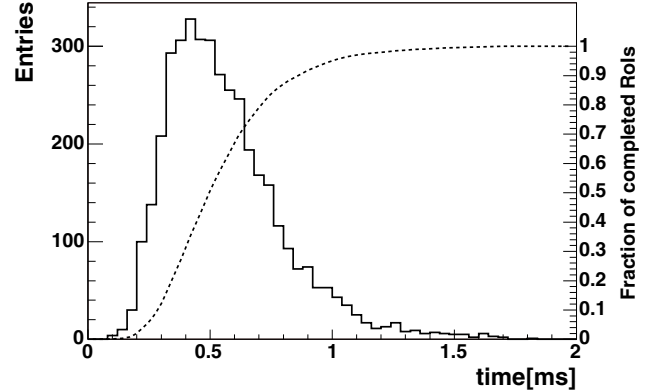
Fig. 6. Inner Detector tracking: total algorithmic execution time for LVL2 single electron reconstruction at initial luminosity; tracking is performed using data from the Pixel and SCT detectors within a \Delta\eta \times \Delta\phi = 0.2 \times 0.2 RoI; results obtained on a 2.8 GHz processor.
