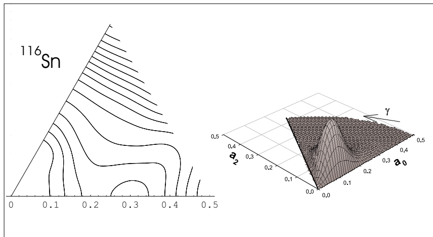
Fig. 3. Same as fig. 2 for the mid shell nucleus ^{116}\text{Sn} ( N = 66 ). Vertical scale for potential V and density \rho^{0,1} are the same as in fig. 2. Maximum value of \rho^{0,1} is 88 for this nucleus.
