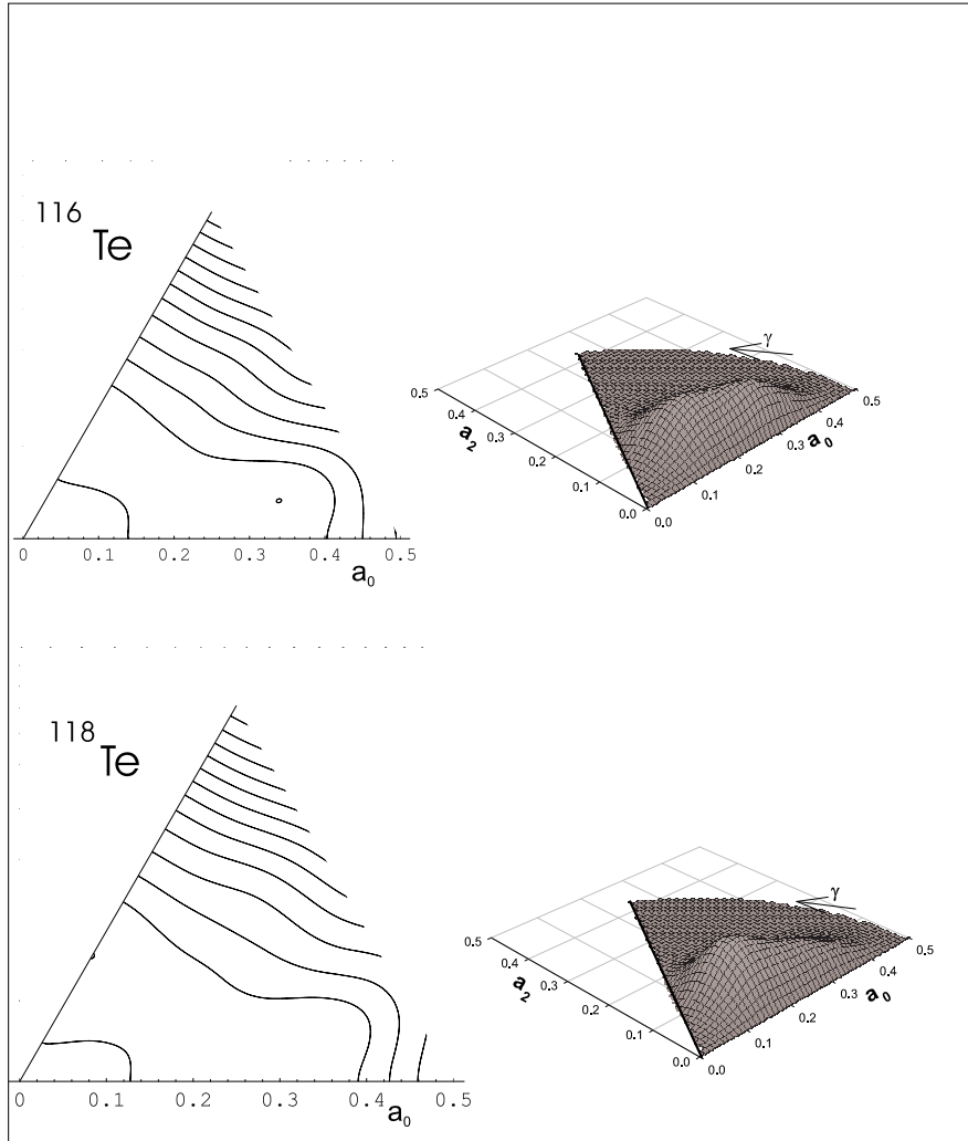
Fig. 7. Same as fig. 2 for ^{116-118}\text{Te} . Vertical scales for potentials V and densities \rho^{0,1} are the same as in fig. 2. Maximum value of \rho^{0,1} is 38 (resp. 45) for ^{116}\text{Te} (resp. ^{118}\text{Te} ).
