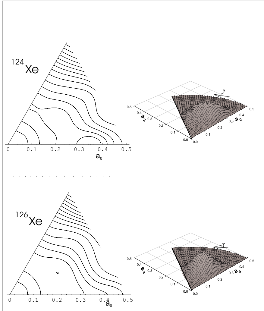
Fig. 8. Same as fig. 2 for ^{124-126}\text{Xe} . Vertical scales in potentials V and densities \rho^{0,1} are the same as in fig. 2. Maximum value of \rho^{0,1} is 46 (resp. 59) for ^{124}\text{Xe} (resp. ^{126}\text{Xe} ).
