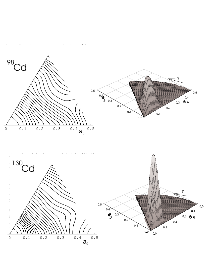
Fig. 2. Potential Energy Surfaces (left hand side) and densities of probability in the ground state (right hand side) -see text- for magic ^{98}\text{Cd} ( N = 50 ) and ^{130}\text{Cd} ( N = 82 ) nuclei. Equipotential lines are separated by 1 MeV. Vertical scales for densities \rho^{0,1} are the same for both nuclei. Maximum value of \rho^{0,1} is 116 (resp. 228) for ^{98}\text{Cd} (resp. ^{130}\text{Cd} ).
