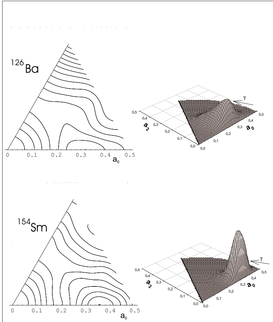
Fig. 4. Same as fig. 2 for the two prolate well deformed nuclei ^{126}\text{Ba} and ^{154}\text{Sm} . Vertical scales for potentials V and densities \rho^{0,1} are the same as in fig. 2. Maximum value of \rho^{0,1} is 65 (resp. 136) for ^{126}\text{Ba} (resp. ^{154}\text{Sm} ).
